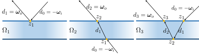
Fig. 6. Example paths of lengths 1, 2 and 3. In our formulation, the exact positions of the vertices do not matter: the z_i only carry information about which interface the vertex occurs on. The first and last in the sequence of directions \mathbf{d}_i map to the incoming and outgoing directions of the underlying BSDF query.
