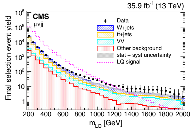
FIG. 7. Data and background event yields after final selections for the \mu\nu jj analysis, as a function of m_{LQ} . “Other background” includes Z/\gamma^* + \text{jets} and single top quark production. The selection criteria for each bin are detailed in Table II. All the bins are correlated, as the events selected for each m_{LQ} are a strict subset of the events selected for the lower mass LQ. The hashed band represents the combined statistical and systematic uncertainty in the full background estimate.
