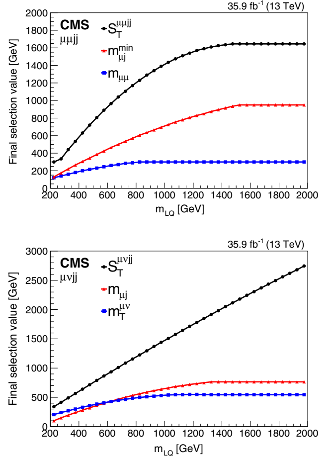
FIG. 4. Lower bounds of the final selection criteria for the three variables for the \mu\mu jj (upper) and \mu\nu jj (lower) channels as a function of scalar m_{LQ} .
