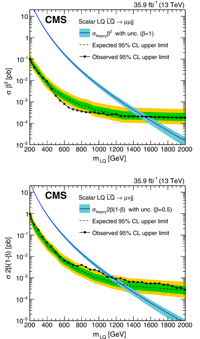
FIG. 8. The expected and observed upper limits at 95% C.L. on the product of the scalar LQ pair production cross section and the branching fractions \beta^2 or 2\beta(1-\beta) as a function of the second-generation m_{LQ} obtained with the \mu\mu jj (upper) or \mu\nu jj (lower) analysis. The solid lines represent the observed limits, the dashed lines represent the median expected limits, and the inner dark green and outer light yellow bands represent the 68% and 95% confidence intervals. The \sigma_{\text{theory}} curves and their blue bands represent the theoretical scalar LQ pair production cross sections and the uncertainties on the cross sections due to the PDF prediction and renormalization and factorization scales, respectively.
