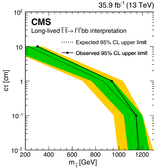
FIG. 10. Expected and observed upper limits at 95% C.L. on the long-lived RPV SUSY \tilde{t} pair production cross section as a function of \tilde{t} mass ( x axis) and lifetime ( y axis). The dashed line and the inner dark green and outer light yellow uncertainty bands represent the median expected limits, and the 68% and 95% confidence intervals, respectively.
