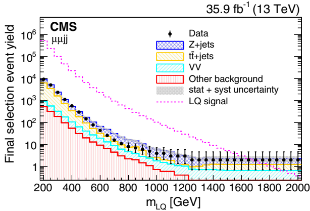
FIG. 6. Data and background event yields after final selections for the \mu\mu jj analysis, as a function of scalar m_{LQ} . “Other background” includes W + \text{jets} and single top quark production. The selection criteria for each bin are detailed in Table I. All the bins are correlated, as the events selected for each m_{LQ} are a strict subset of the events selected for the lower mass LQ. The hashed band represents the combined statistical and systematic uncertainty in the full background estimate.
