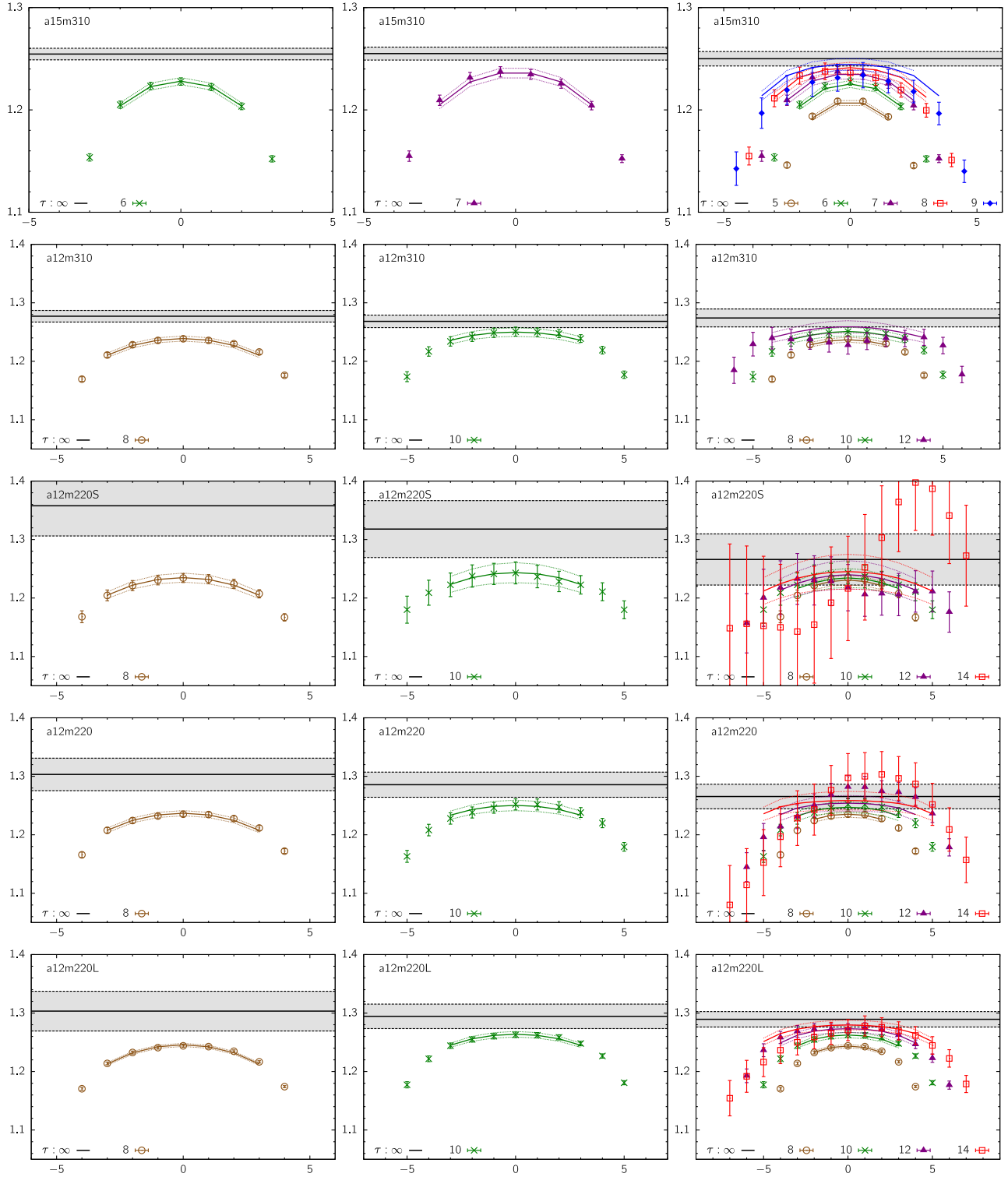
FIG. 9. Comparison between the 2^* and 3^* fits to the axial charge g_A^{u-d} data from the a \approx 0.15 fm (top row) and a \approx 0.12 fm (bottom four rows) ensembles. The results of the fits are summarized in Table XIII along with the number of points t_{\text{skip}} skipped. The first two columns show 2^* fits to data versus t at a single value of \tau , while the third panel shows the 3^* fit using data at multiple values of \tau . The labels give the ensemble ID, and the values of \tau used in the fits. The \tau \rightarrow \infty value is given by the grey band in each panel.
