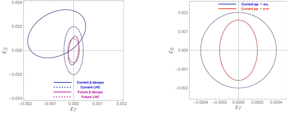
FIG. 8. Current and projected 90% C.L. constraints on \epsilon_S and \epsilon_T defined at 2 GeV in the \overline{\text{MS}} scheme. (Left) The beta-decay constraints are obtained from the recent review article, Ref. [81]. The current and future LHC bounds are obtained from the analysis of the pp \rightarrow e + \text{MET} + X . We have used the ATLAS results [82], at \sqrt{s} = 13 TeV and integrated luminosity of 36 \text{ fb}^{-1} . We find that the strongest bound comes from the cumulative distribution with a cut on the transverse mass at 2 TeV. The projected future LHC bounds are obtained by assuming that no events are observed at transverse mass greater than 3 TeV with an integrated luminosity of 300 \text{ fb}^{-1} . (Right) Comparison of current LHC bounds from pp \rightarrow e + \text{MET} + X versus pp \rightarrow e^+e^- + X .
