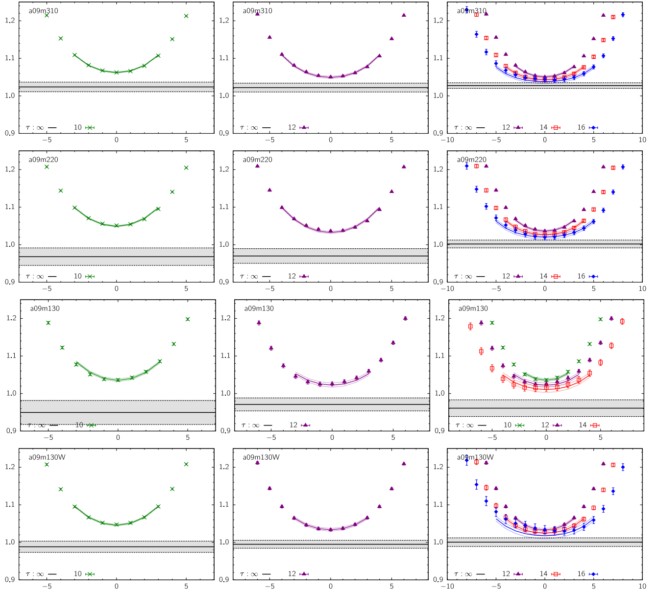
FIG. 16. Comparison between the 2* and 3* fits to the tensor charge g_T^{\mu-d} data from the a \approx 0.09 fm ensembles. The rest is the same as in Fig. 9.
