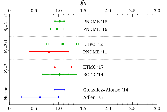
FIG. 6. A summary of results for the isovector scalar charge, g_S^{u-d} , for N_f = 2, 2 + 1 , and 2 + 1 + 1 flavors. The lattice results are from: PNDME'18 (this work); PNDME'16 [3]; LHPC'12 [71]; PNDME'11 [13]; ETMC'17 [36]; and RQCD'14 [59]. The estimates based on the conserved vector current and phenomenology are taken from Gonzalez-Alonso'14 [49] and Adler'75 [72]. The rest is the same as in Fig. 5.
