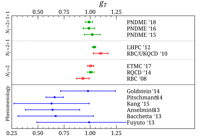
FIG. 7. A summary of results for the isovector tensor charge, g_T^{u-d} , for N_f = 2, 2 + 1 , and 2 + 1 + 1 flavors. The lattice and phenomenology results are quoted from: PNDME'18 (this work); PNDME'16 [3]; PNDME'15 [1]; LHPC'12 [71]; RBC/UKQCD'10 [73]; ETMC'17 [36]; RQCD'14 [59]; and RBC'08 [62]. The phenomenological estimates are taken from the following sources: Kang'15 [74]; Goldstein'14 [75]; Pitschmann'14 [76]; Anselmino'13 [77]; Bacchetta'13 [78]; and Fuyuto'13 [79]. The rest is the same as in Fig. 5.
