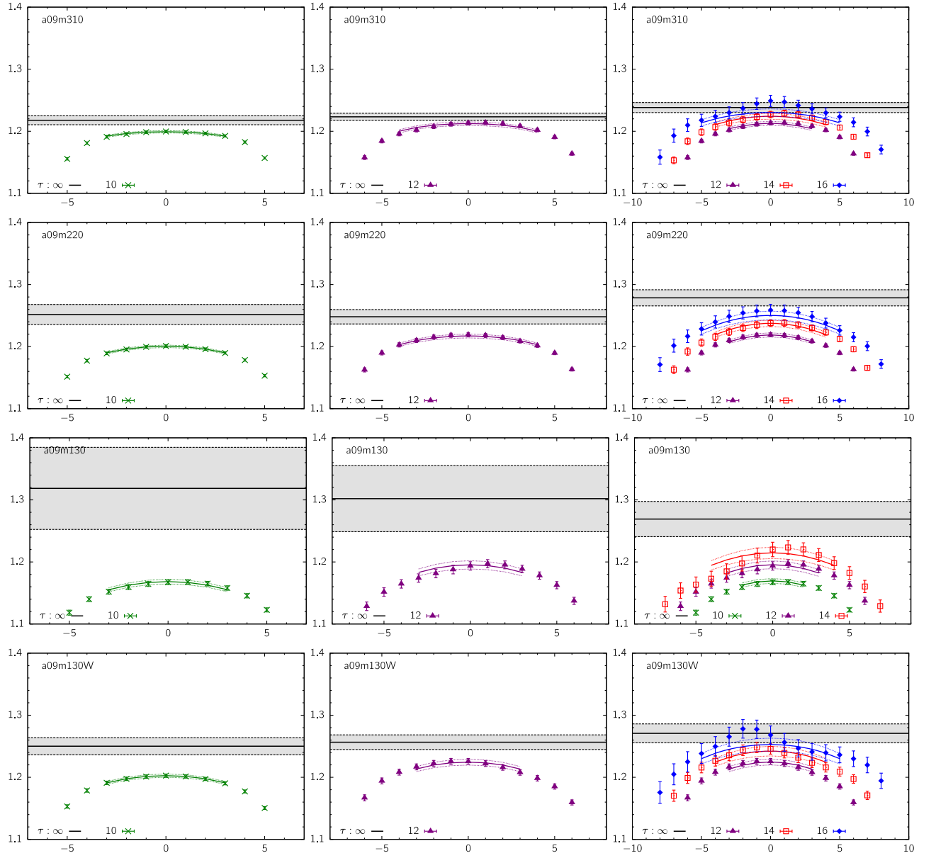
FIG. 10. Comparison between the 2* and 3* fits to the axial charge g_A^{\mu-d} data from the a \approx 0.09 fm ensembles. The rest is the same as in Fig. 9.
