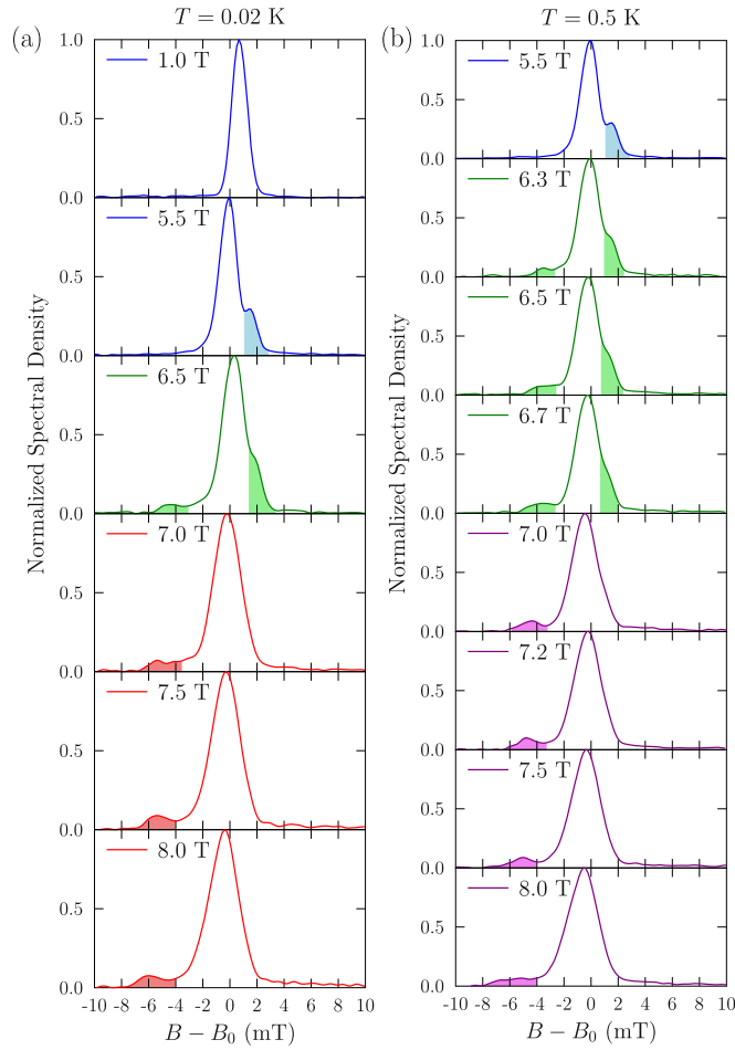
Figure 2. Fourier transform TF \mu^+ SR spectra measured for (Hpip) _2 CuBr _4 at fixed temperatures of (a) T = 0.02 K and (b) T = 0.5 K. Colours refer to figure 1(a) and shading highlights the satellite peaks.
