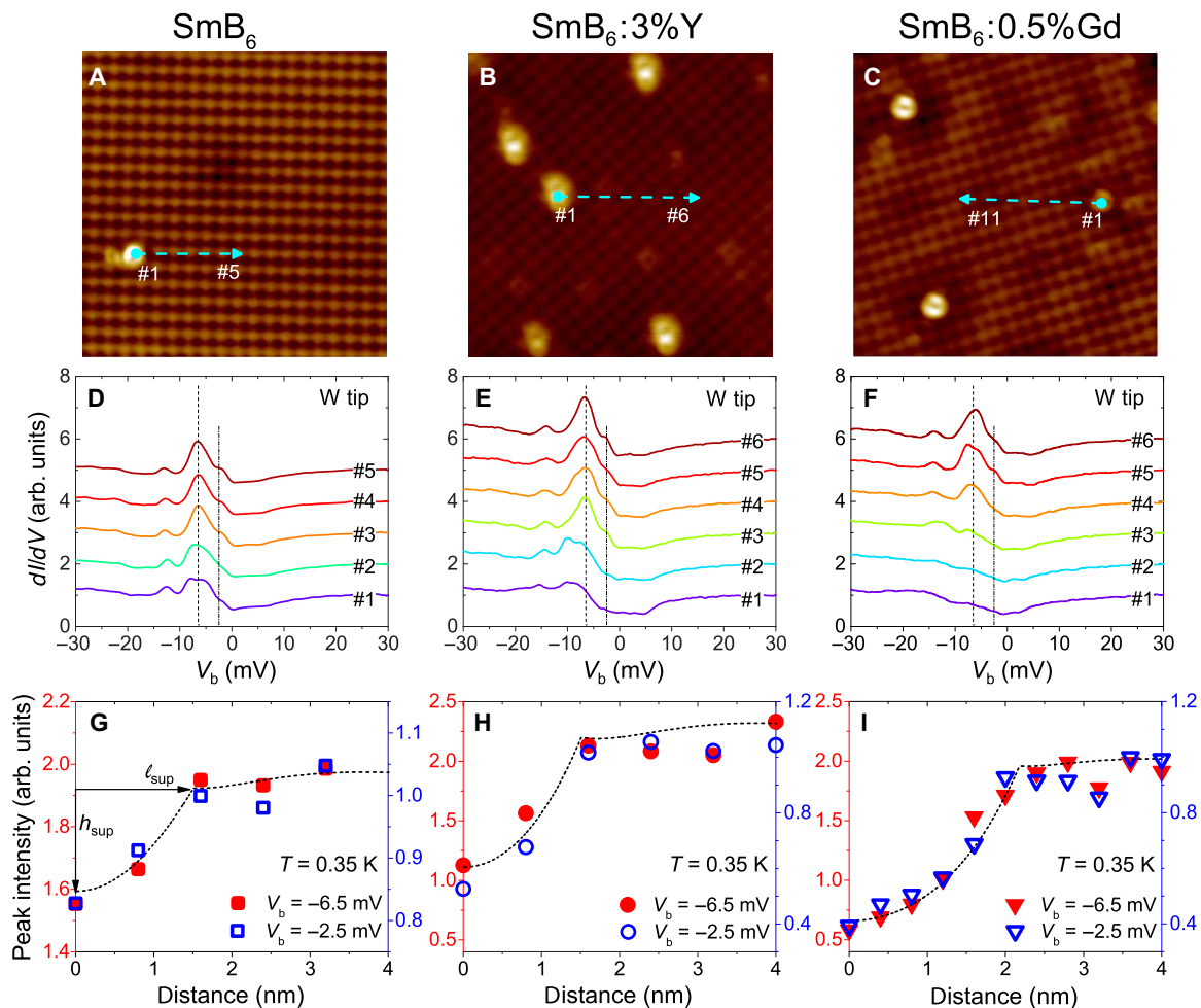
Fig. 2. Influence of impurities on spectroscopic results. (A to C) Topographies (8 nm by 8 nm) of pure \text{SmB}_6 as well as \text{SmB}_6:3\%\text{Y} and \text{SmB}_6:0.5\%\text{Gd} . The cyan arrows indicate the ranges and directions of STS measurements around the impurities. (D to F) dI/dV curves of the three samples measured at 0.35 K and zero field. The curves are measured at positions with increasing distance from the impurity (the impurities are located at #1) along the arrows in (A) to (C), correspondingly ( V_b = 30 mV; I_{sp} = 100 pA). (G to I) dI/dV values at V_b = -6.5 mV (red) and -2.5 mV (blue) with increasing distance from the impurity (impurities are located at 0). The black dashed lines are fits according to the model (see text S6). h_{sup} and \ell_{sup} indicate the suppression of peak intensity at the impurity and its lateral extent, respectively.
