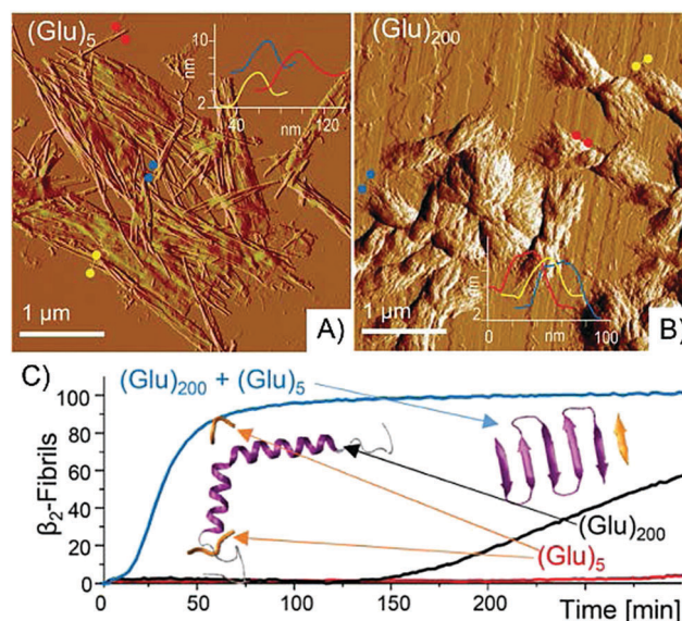
Fig. 16 The influence of chain lengths on the formation of amyloid fibrils. (A and B) AFM tapping-mode images of \text{PLG}_5 (A) and \text{PLG}_{200} (B). Scale bar = 1 \mu\text{m} . The cross sections of selected fibrillary specimens are shown in the insets. The thickness of the fibril is independent of the chain length of PLG. Both samples are longer than the critical length to form amyloid fibrils. As a result, long, straight, and unbranched fibrils are observed in both images. Reprinted with permission from ref. 167. Copyright 2015 American Chemical Society. (C) Fibrillization kinetics of \text{PLG}_5 and \text{PLG}_{200} , and their mixtures at 40^\circ\text{C} . By mixing the short PLG with the long PLG, the fibrillization rate is greatly enhanced. Reprinted with permission from ref. 168. Copyright 2016 American Chemical Society.
