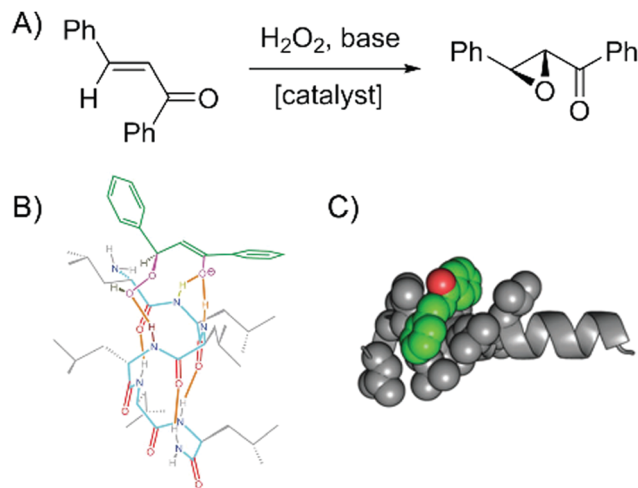
Fig. 20 Juliá-Colonna epoxidation and the proposed reaction mechanism. (A) Synthetic scheme showing the epoxidation of enone in the presence of polypeptide catalysts. (B) The structure of the complex with PLLeu and 3-hydroxy-chalcone enolate. The enantioselectivity originates from the hydrogen bonding motif as well as the helical conformation of PLLeu. Reprinted with permission from ref. 231. Copyright 2004 Royal Society of Chemistry. (C) Interaction of trans -chalcone with PLLeu. PLLeu blocks are presented as grey cartoons and the PLLeu side chains interacting with trans -chalcone are presented as spheres. The trans -chalcone substrate fits within the hydrophobic, chiral grooves of PLLeu. Reprinted with permission from ref. 224. Copyright 2017 Royal Society of Chemistry.
