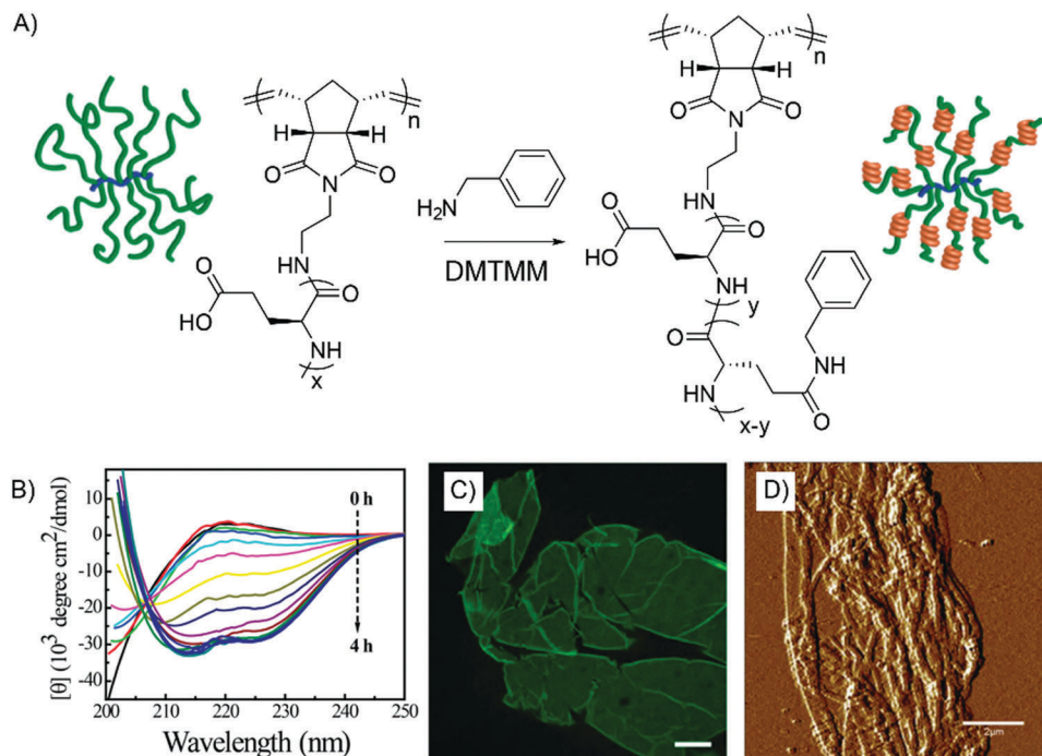
Fig. 12 Chemical modification induced self-assembly of polypeptide-based copolymers. (A) Scheme showing the modification of PN-g-PLG by benzylamine and the accompanying secondary structure change from random coils to \alpha -helices. 4-(4,6-Dimethoxy-1,3,5-triazin-2-yl)-4-methylmorpholinium chloride (DMTMM) is used as the coupling agent. (B) CD spectra revealing the time progress of the conformational changes in PLGs after PN 10 -g-PLG 102 reacts with benzylamine (0.5 mg mL -1 polymer, pH = 7, rt). The amidation reaction converts charged PLG residues into neutral residues, leading to coil-to-helix transitions. (C and D) Confocal microscopy (C, stained with Thioflavin T) and AFM amplitude (D) images of thin membranes assembled from benzylamine substituted PN 10 -g-PLG 102 samples. Scale bar = 20 \mu m for (C) and 2 \mu m for (D). Reprinted with permission from ref. 146. Copyright 2017 American Chemical Society.
