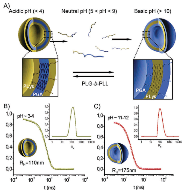
Fig. 13 pH-Responsive, reversible assembly and disassembly of copolypeptides. (A) Scheme showing the pH-responsive self-assembly of PLG- b -PLL into a vesicular morphology. At pH < 4, the PLG segment forms a neutral \alpha -helical structure and remains in the interlayer, while the charged PLL block adopts a random coil conformation and remains in the corona. The interlayer and corona are reversed at pH > 10. (B and C) Auto correlation functions ( 90^\circ ) of PLG 15 - b -PLL 15 at pH = 3 (B) and pH = 12 (C). The corresponding R_H distributions are shown in the insets. Reprinted with permission from ref. 148. Copyright 2005 American Chemical Society.
