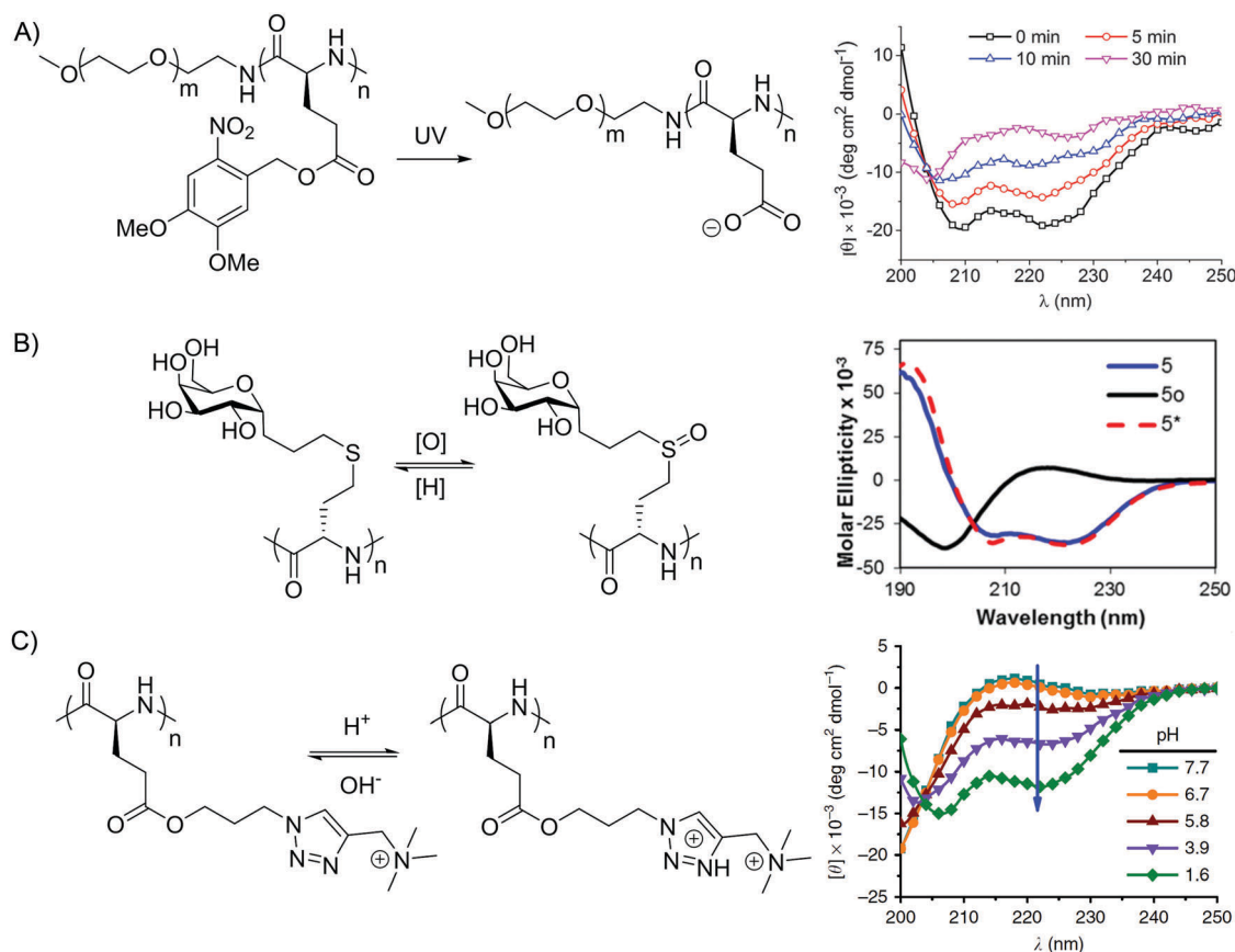
Fig. 3 Trigger-responsive helix-coil transition of polypeptides. (A) Chemical structure and UV-triggered helix-to-coil transition of PDMNBLG. Upon UV irradiation, the cleavage of side-chain esters leads to the exposure of negative charges, which destabilizes the \alpha -helical conformation due to charge repulsion. Reprinted with permission from ref. 70. Copyright 2015 Royal Society of Chemistry. (B) Chemical structure and redox-responsive, reversible helix-coil transition of sugar-based poly(L-homocysteine) derivatives. The oxidation of side-chain thioethers to sulfoxides increases the polarity and disrupts the hydrophobic interaction of side chains, resulting in a helix-to-coil transition. 5 was first oxidized to 5o, which was then reduced back to 5*. Reprinted with permission from ref. 74. Copyright 2014 American Chemical Society. (C) Chemical structure and pH-responsive, reversible helix-coil transition of triazole-based polypeptides. The protonation/deprotonation of side-chain triazoles alters their hydrogen bonding pattern, leading to reversible conformational changes of the polypeptides. Reprinted with permission from ref. 53. Copyright 2017 Springer Nature.
