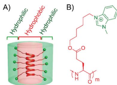
Fig. 19 Scheme illustration (A) and the chemical structure (B) of radially amphiphilic antimicrobial polypeptides, PHLG-BIm. The radial structure facilitates the interactions with bacterial membranes, while reducing non-specific interactions with eukaryotic cell membranes. Reprinted with permission from ref. 65. Copyright 2015 National Academy of Sciences.
