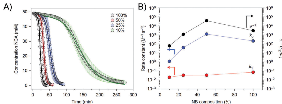
Fig. 22 Kinetic modeling of the brush polymerization. (A) Kinetic data (circles) obtained from the polymerization of BLG-NCA with PNB- r -PPH macroinitiators are fit with the two-stage kinetic model (solid lines). (B) Extracted rate constants for the primary nucleation stage ( k_1 ) and the second elongation stage ( k_2 ). The density of initiating groups has a greater effect on k_2 , which correlates the interaction between macrodipoles with the cooperative growth of polypeptides. Reprinted with permission from ref. 237. Copyright 2017 Springer Nature.
