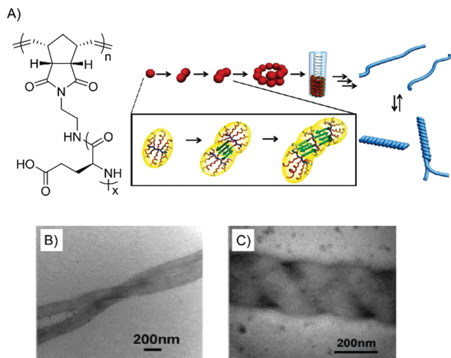
Fig. 9 Topology induced anti-parallel \beta -sheets. (A) Schematic illustration of PN-g-PLG forming tubular superstructures. The interactions between PLG chains from brush-like PN-g-PLG polymers result in the formation of anti-parallel \beta -sheets, which further induces helical tubular superstructures. (B and C) TEM images of the helical tubular structures from PN 11 -g-PLG 101 . Scale bar = 200 nm. Reprinted with permission from ref. 121. Copyright 2011 American Chemical Society.
