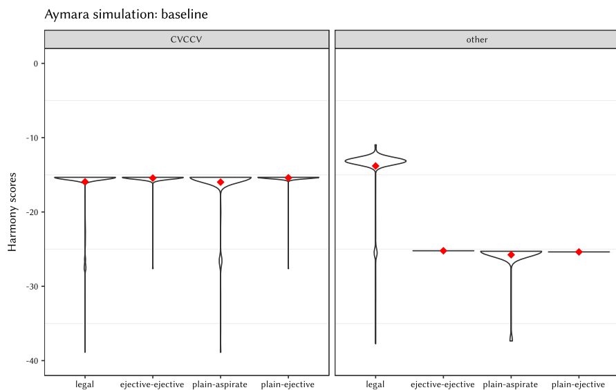
Fig. 4 Aymara: Harmony scores for nonce words, baseline grammar
