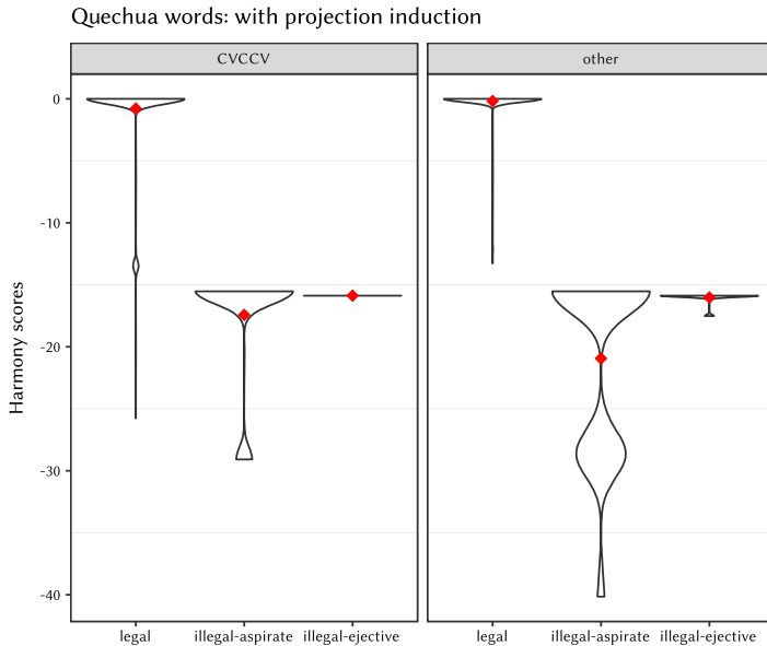
Fig. 3 Quechua: Harmony scores for nonce words, simulation with projection induction
