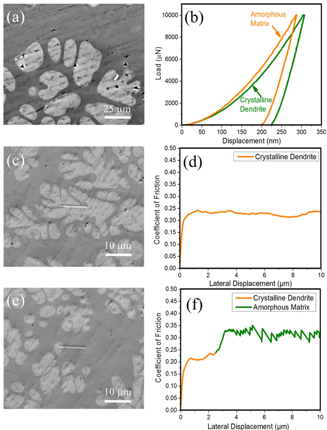
Figure 3. Phase-specific nano-indentation results: (a) SEM image showing indentations on bright crystalline dendrite and dark amorphous matrix and (b) load versus displacement curves obtained on the respective phases; (c) SEM image of scratch test performed on crystalline dendrite and (d) the corresponding coefficient of friction; (e) Scratch on both crystalline and amorphous phases and (f) the corresponding coefficient of friction for both phases. The friction coefficient was higher for the amorphous matrix and had a saw-tooth type profile compared to a smooth/uniform value for the crystalline dendrite.
