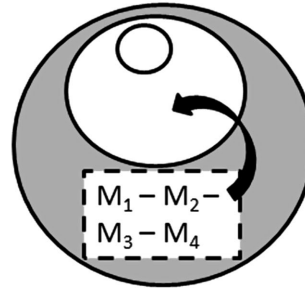
Figure 4. Two alternative accounts for the functioning of the covert retrieval mechanism. M, memory item; in this example, participants would be attempting to remember a four-item list. On the left, all four items are currently available in the central component of WM, and refreshing them in sequence maintains them as active and available. On the right, prior to covert retrieval, no task-relevant information is within the central component of WM, and the list must be “reloaded” from longer term memory stores.
