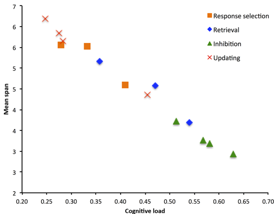
Figure 3. Mean WM spans as a function of the approximate cognitive load induced by a variety of tasks involving different executive functions such as response selection and retrieval, 47 updating and inhibition. 35
