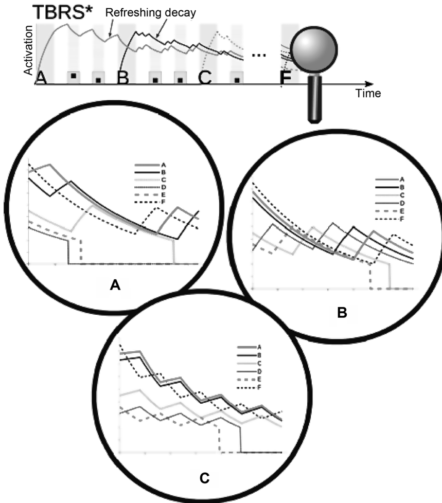
Figure 1. This diagram illustrates the evolution of the item/position activation values in the TBRs* model in a fictional task in which there are six to-be-recalled letters (ABCDEF) and two distractors interleaved after each letter for which a location judgment task has to be performed. The first item to be maintained is A. The light gray area represents the encoding step during which the activation of A is increased. The next white area represents the time devoted to refreshing items. Since there is only one item (A) encoded so far in WM, the activation value continues to increase until a distracting episode occurs (horizontal hatching area); activation then decays. The task then alternates between free time (refreshing) and distractors (decay) until a new item, B, occurs. During the free time following the encoding of B, as well as during the free time following a concurrent processing episode, the two items (A and B) are refreshed in turn: when one is refreshed, the other one decays, and so on until the end of the series. This evolution of activations values derives from the default cumulative schedule of refreshing implemented by Oberauer and Lewandowsky. 20 The magnifying circle at the right side of the diagram emphasizes the time course of the respective activation of the six items during a refreshing phase as a function of the three schedules: (A) cumulative, (B) least-activated first, and (C) expanded focus of attention. 8
