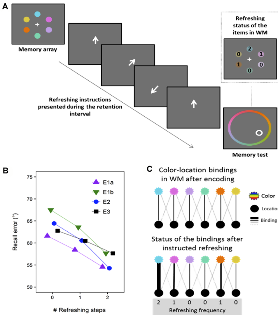
Figure 2. (A) Flow of events in the refreshing visual WM task employed by Souza et al. 11 Participants encoded six colored dots, and at the end of a brief interval were asked to reproduce the color of one dot (marked by a white circle) using a color wheel. During maintenance, cues (arrow) instructed participants to think of WM items (refreshing instruction). WM items were cued 0, 1, or 2 times (see inset). (B) Error (distance in degrees on the color wheel) in reproducing the test item's color as a function of the number of refreshing steps this item received in the four experiments reported by Souza et al. 11 (C) Schematic illustration of the effect of refreshing on the bindings between content (represented here by color) and the context (spatial location on the screen).
