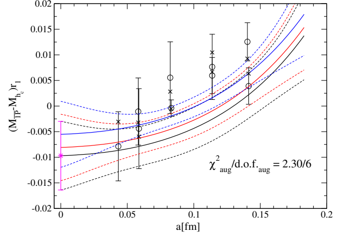
FIG. 6. Chiral and continuum fit for the P-wave hyperfine splitting. The black circles denote the lattice data. Curves for physical (black), 0.1m_s (red), and 0.2m_s (blue) light-quark masses are plotted. The black crosses show the fit results evaluated at the lattice parameters of the gauge ensemble. The magenta symbol indicates the result in the combined chiral and continuum limit.
