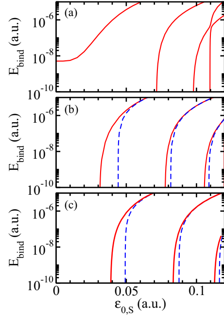
FIG. 2. Binding energy E_{\text{bind}} for (a) ^4\text{He}-^4\text{He} , (b) ^3\text{He}-^4\text{He} , and (c) ^3\text{He}-^3\text{He} as a function of the field strength \epsilon_{0,S} . The solid lines show the binding energy of states that are even in z while the dashed lines show the binding energy of states that are odd in z . Note that the binding energy is shown on a logarithmic scale that covers five orders of magnitude.
