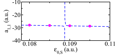
FIG. 4. Enlargement of the scattering length a_{1,1} for {}^3\text{He}-{}^4\text{He} in the vicinity of a resonance. The data and symbol/line styles are the same as in Fig. 3(c).
