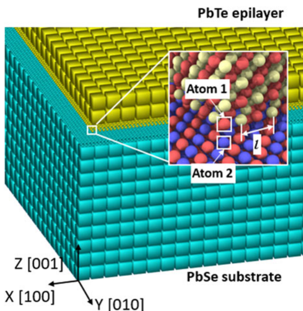
Figure 6: Schematic diagram of the bilayer simulation model. The X , Y , and Z directions are along [100] , [010] , and [001] lattice directions, respectively. The inset shows an exploded view of the atomic structure at the corner of the PbTe layer. Red spheres denote Pb atoms, blue spheres denote Se atoms, and yellow spheres denote Te atoms. The relative position of the epilayer with respect to the substrate is defined as the relative position of atom 1 with respect to atom 2. In this figure, the relative position of atom 1 with respect to atom 2 is 0 along the X and Y directions. l denotes the distance of adjacent unit cells in PbTe layer along the X and Y directions in initial bilayer models.
