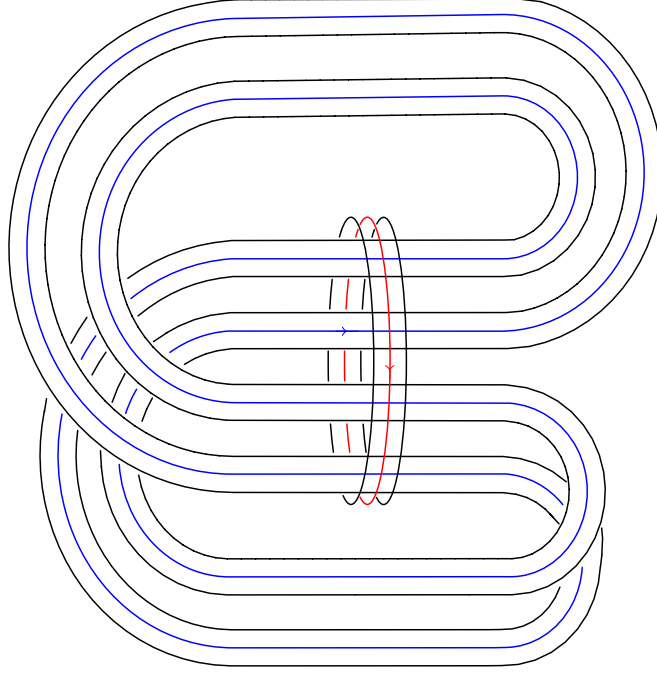
Figure 2: S = \{1, 2, 3, 4\}, C_1 = (1, 2, 3, 4), C_2 = (1, 3, 2, 4)
