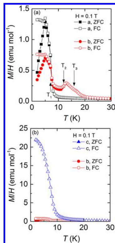
Figure 4. (a) ZFC and FC temperature-dependent magnetization data for H|| a and H|| b . The three magnetic ordering temperatures are marked with the arrows. (b) ZFC and FC magnetization for H|| b and H|| c . Here the M ( T ) data for H|| b are repeated for comparison.
