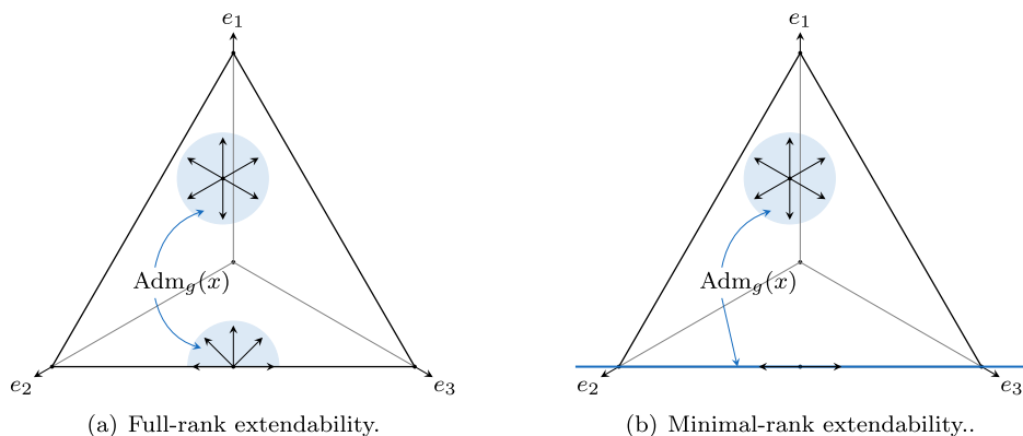
Fig. 2. Admissible cones under the Euclidean and Shahshahani metrics. For x \in \mathcal{X}^\circ , we have \text{Adm}_g(x) = \text{TC}_{\mathcal{X}}(x) . For x \in \text{bd}(\mathcal{X}) , we still have \text{Adm}_g(x) = \text{TC}_{\mathcal{X}}(x) in the Euclidean case, but the Shahshahani metric can only be extended to the tangent space \text{Adm}_g(x) = \text{T}_{\mathcal{X}}(x) .
