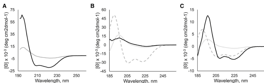
FIGURE 5 Structure and orientation of GWALP23 in DSPC/DOPC/choLd and Lo. (A) CD spectra of GWALP23 in Ld phase (black) and Lo phase (gray) are shown. (B and C) OCD spectra of GWALP23 in hydrated stacked Ld (B) and Lo (C) lipid bilayers are shown. The dotted and dashed lines correspond to theoretical OCD spectra for an ideal \alpha -helix aligned parallel (dotted) and perpendicular (dashed) to the membrane normal; the spectra correspond to trans-membrane and peripheral helical peptides, respectively. The significant difference in helicity (7% versus 56%) resulted in the variation in the theoretical curves for GWALP23 in Ld (B) and Lo (C).
