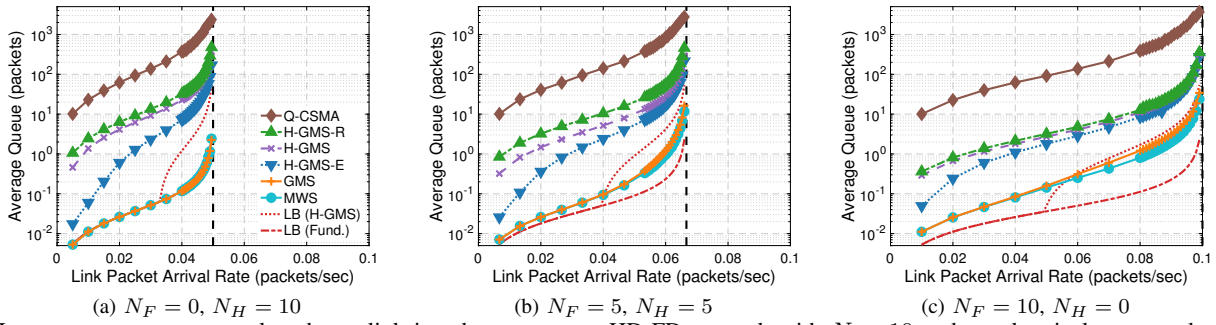
Fig. 1: Long-term average queue length per link in a heterogeneous HD-FD network with N = 10 and equal arrival rates, under varying number of FD users, N_F : (a) N_F = 0 , (b) N_F = 5 , and (c) N_F = 10 . Both the fundamental and improved lower bounds on the delay are also plotted according to (7) and (8). The capacity region boundary in each HD-FD network is illustrated by the vertical dashed line.
