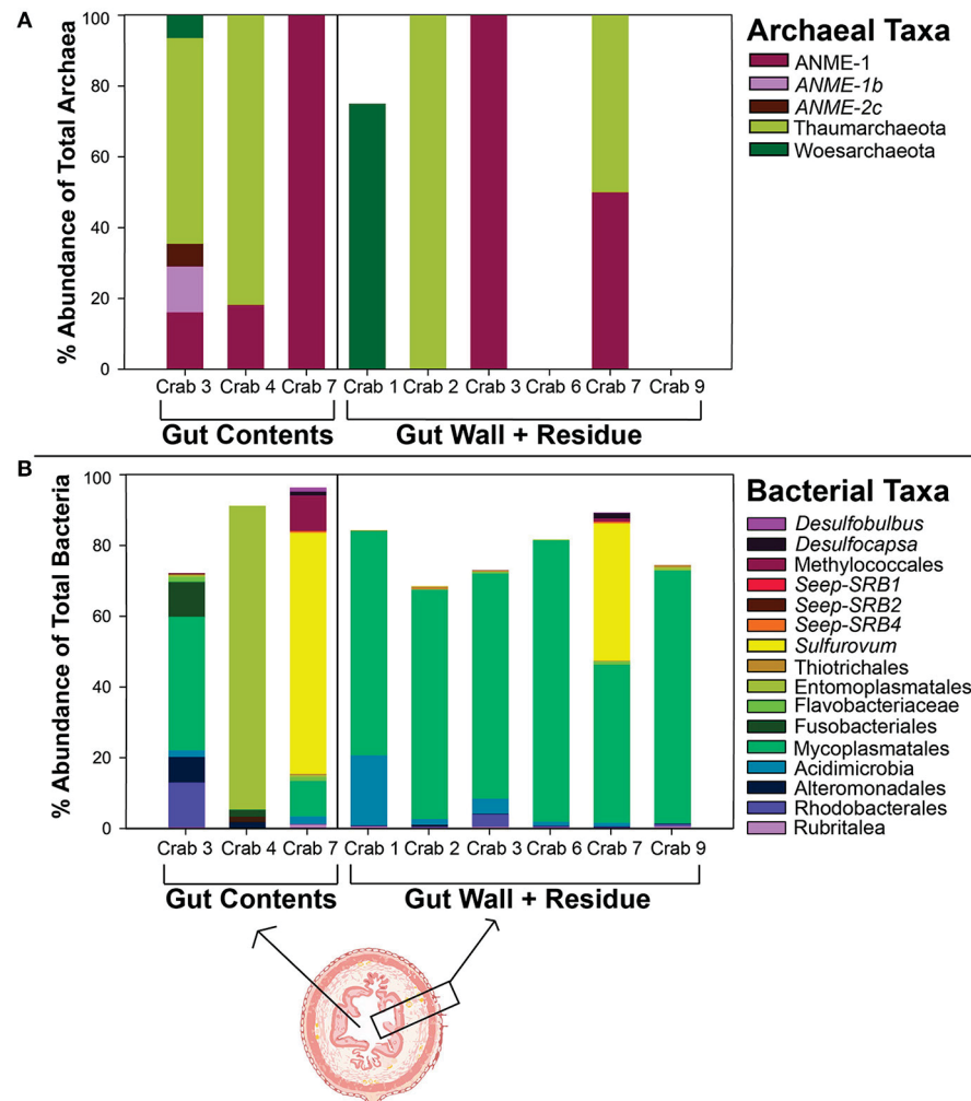
FIGURE 4 | The percent abundance of the (A) archaea and (B) bacteria isolated from the gut contents and gut wall and residue of C. tanneri . In (A) only the five most dominant archaeal groups are shown, and in (B) the 16 most dominant bacterial groups are shown. The order is given for the bacterial and archaeal groups, except in italicized instances when genus is given for clarity.
