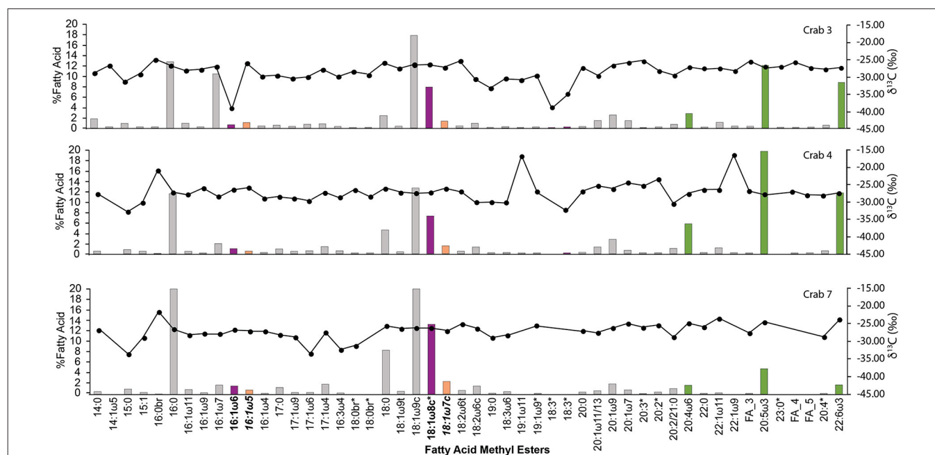
FIGURE 3 | The fatty acid (FA) distribution and carbon isotope composition of FAs extracted from C. tanneri muscle tissue. Left y-axis and bars represent percentage of FA, while right axis and points are the isotopic composition. Pink bars with FAs in bold have been associated with methanotrophic bacteria, orange bars with FAs in italic bold have been associated with sulfate reducing bacteria, and green bars are essential fatty acids linked to photosynthetic sources. Asterisks represent instance where FA compounds were inferred from mass spectra.
