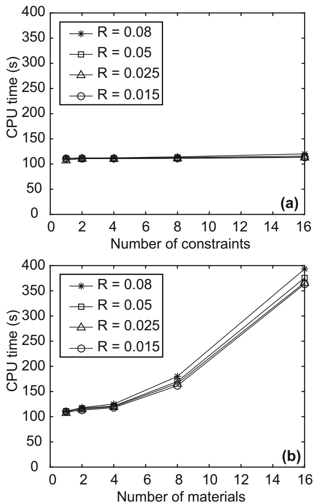
Fig. 7 CPU time (seconds) for the MBB beam problem with a 300 \times 100 orthogonal mesh run for 200 iterations: a a single candidate material controlled by a varying number of local volume constraints on sub-regions of the domain; and b a single global volume constraint controlling a varying number of candidate materials
