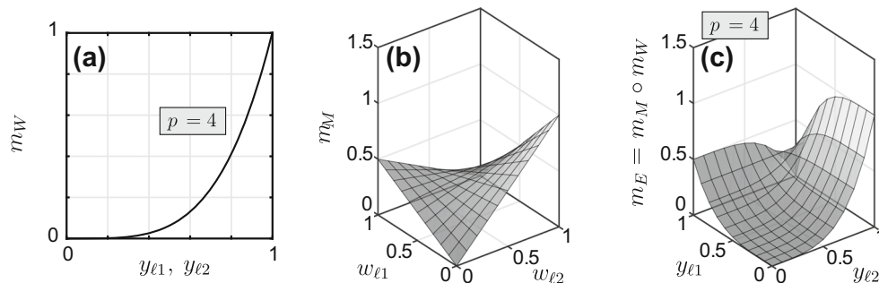
Fig. 3 Material interpolation functions for two candidate materials ( E_1 = 0.5 , E_2 = 1 ) in element \ell considering SIMP with p = 4 and \varepsilon = 0 : a m_W (see (19)); b m_M (see (20)); and c m_E = m_M \circ m_W
