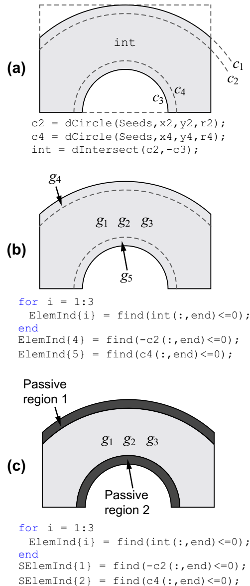
Fig. 2 Constraint specification: a curved beam domain and code needed to generate the distance values required to define the constraints and/or passive regions; b constraint specification and code needed to assemble ElemInd; and c constraint and passive region specification and code needed to assemble ElemInd and SElemInd
