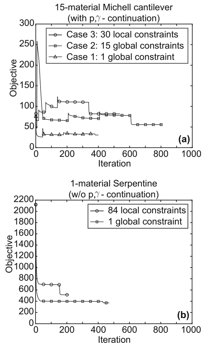
Fig. 20 Convergence plots: a 15-material Michell cantilever with continuation on the material interpolation parameters and with filter reduction in the final continuation step and b 1-material serpentine without continuation on the material interpolation parameters and with filter reduction after convergence
