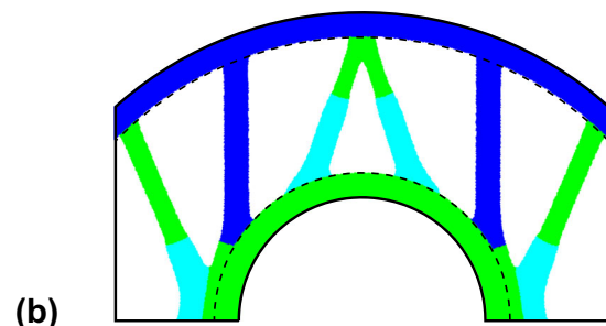
Fig. 16 Curved beam problem: a domain, boundary conditions, constraint specification, and passive region specification; and b optimized design (color online)
