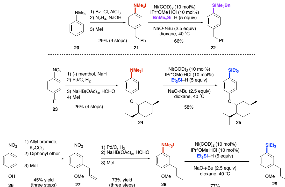
Scheme 1 Synthetic application of aryl trialkylammonium salt
