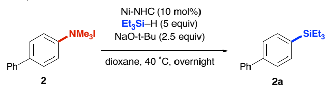
Scheme 2 Comparison an in situ formed and air-tolerant nickel complex
