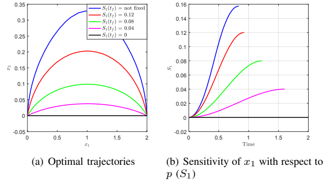
Fig. 5: Results obtained for the Zermelo's path optimization problem - Sensitivity of the final state with respect to the uncertain parameter is fixed
