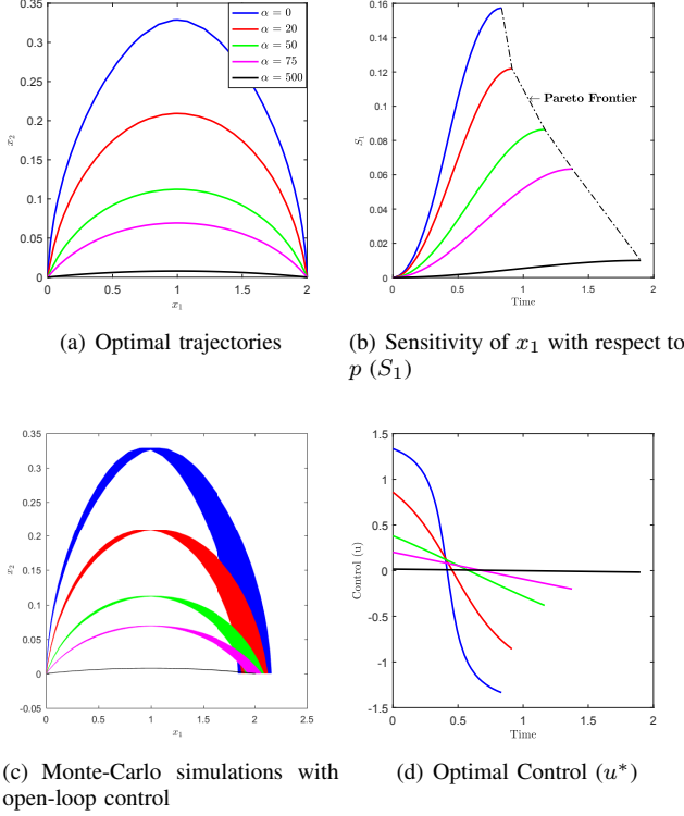
Fig. 3: Results obtained for the Zermelo's path optimization problem with final state desensitization
