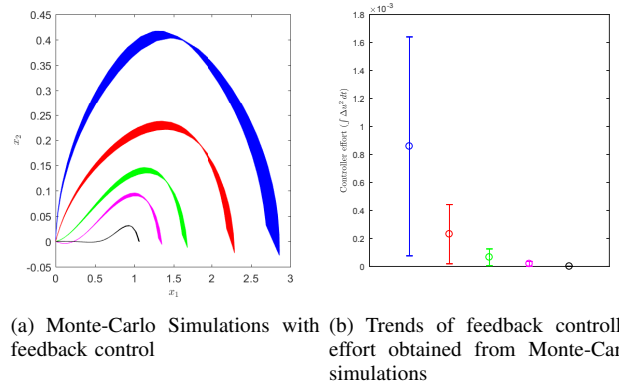
Fig. 2: Results for trajectory desensitization with feedback control
