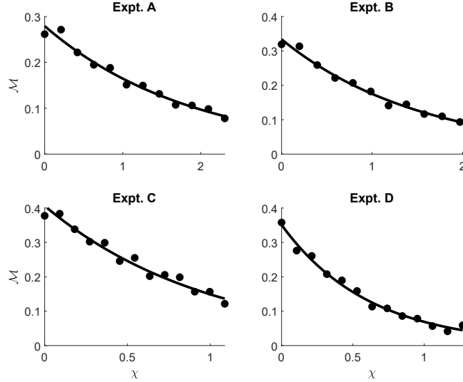
Figure 4: Plots of (dimensionless) \mathcal{M} versus (dimensionless) \chi for the four experiments. bluePlots of dimensionless mass, \mathcal{M} , versus dimensionless distance down the tank, \chi , for the four experiments. The dots correspond to experimental measurements and the curves are the best-fit exponentials.
