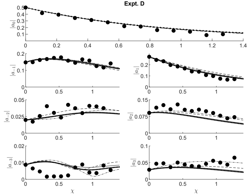
Figure 3: Plots of the nondimensional amplitudes of the carrier wave, blue |a_0| , and the three most energetic sideband pairs, blue |a_{\pm j}| , versus nondimensional distance down, blue \chi , the tank for Expt D. The large dots correspond to experimental measurements, the dashed curves correspond to dNLS, the solid curves correspond to vDysthe, the dash-dot curves correspond to optimized IS, and the dotted curves correspond to dGT.
