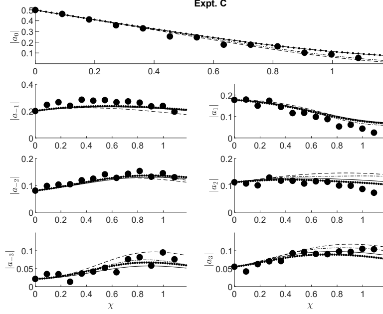
Figure 2: Plots of the nondimensional amplitudes of the carrier wave, blue |a_0| , and the three most energetic sideband pairs, blue |a_{\pm j}| , versus nondimensional distance down the tank, blue \chi , for Expt C. The large dots correspond to experimental measurements, the dashed curves correspond to dNLS, the solid curves correspond to vDysthe, the dash-dot curves correspond to optimized IS, and the dotted curves correspond to dGT.
