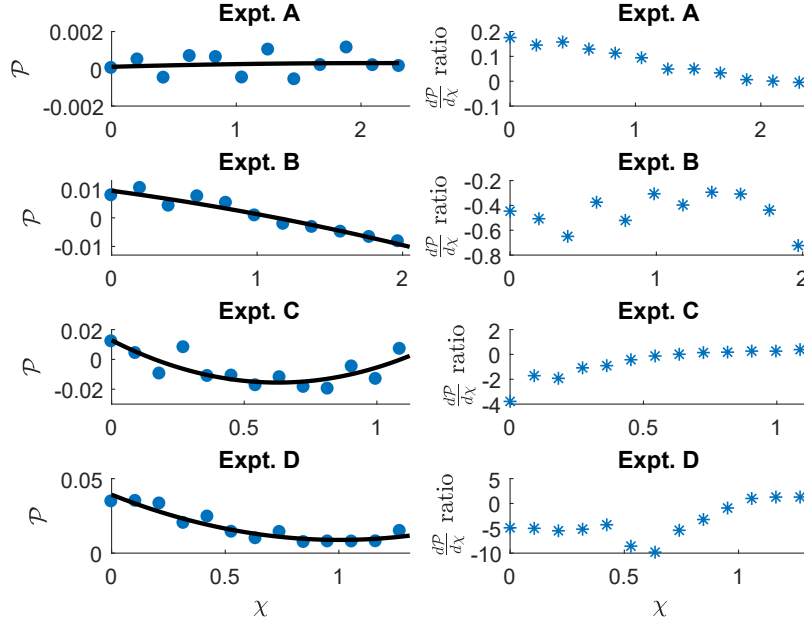
Figure 8: The first column contains plots of the linear momentum, \mathcal{P} , versus dimensionless distance down the tank, \chi , for each experiment. The dots correspond to experimental measurements and the curves are the best quadratic fits. The second column contains plots of the ratio of experimentally determined S , blue see (21), and \frac{d\mathcal{P}}{d\chi} estimated using the quadratic fits shown in the first column.
