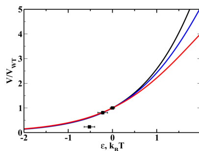
Figure 7. Normalized velocities of kinesin molecules as a function of the parameter \varepsilon . The WT kinesin corresponds to \varepsilon = 0 k_B T . The lines represent theoretical predictions (black curve is for F = 0 \text{pN} , blue curve is for F = 4 \text{pN} , red curve is for F = 7 \text{pN} ). Symbols are experimental data from ref 22. To the left on the graph, the probability of open conformation of the ATP-binding pocket increases, and to the right, it decreases.
