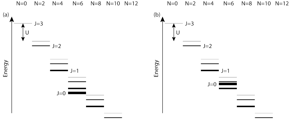
Fig. 2. Schematic of a pseudospin tower for the attractive Hubbard model. (a) Pseudospin tower for |\Lambda| = 6 on a lattice with N_A = N_B and (b) pseudospin tower for |\Lambda| = 6 on a lattice with N_A = 2 and N_B = 4 . The energy levels are plotted on the vertical axis and the electron number on the horizontal. We only show the lowest energy level for each pseudospin for a given number of electrons. The thickness of the line denotes the pseudospin value, as labeled in the figure. The energy decreases by exactly -|U| as the electron number increases by 2, as shown in the figure. In panel (b), the minimal energy state has J = 1 for 4, 6, and 8 electrons due to the partial pseudospin tower, which occurs on a Lieb lattice.
