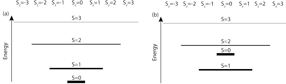
Fig. 3. Schematic of a spin tower at half-filling for the repulsive Hubbard model. (a) Spin tower for |\Lambda| = 6 on a lattice with N_A = N_B and (b) spin tower for |\Lambda| = 6 on a lattice with N_A = 2 and N_B = 4 . The energy levels are plotted on the vertical axis and the z -component of the electron spin on the horizontal. We only show the lowest energy level for each total spin quantum number. The thickness of the line denotes the spin value, as labeled in the figure. In panel (b), the minimal energy state has S = 1 for S_z = 0, \pm 1 due to the partial spin tower, which occurs on a Lieb lattice.
