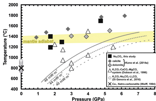
Fig. 1. Diagram showing temperatures and pressures set for the experiments of this study compared to previous studies, plotted along with the mantle adiabat and Archean cratonic geotherms.
