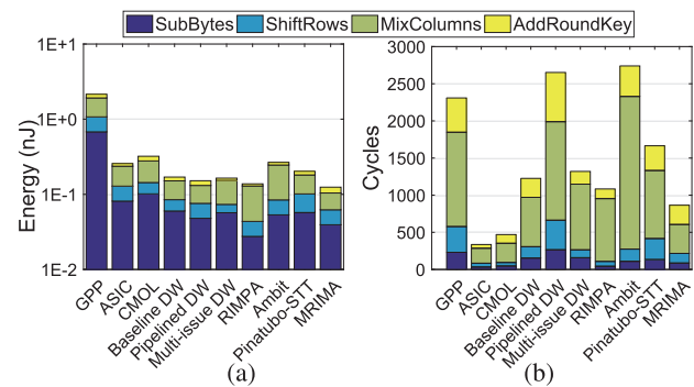
Figure 20: Breakdown of (a) Energy consumption and (b) Delay of different AES implementations.
