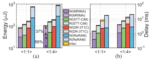
Figure 17: Break-down of (a) Energy and (b) Delay of four PIM platforms.
