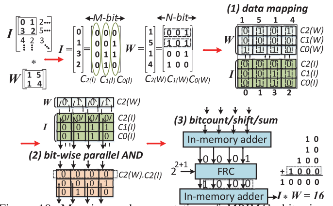
Figure 10: Mapping and computation of MRIMA 's bit-wise convolver.
