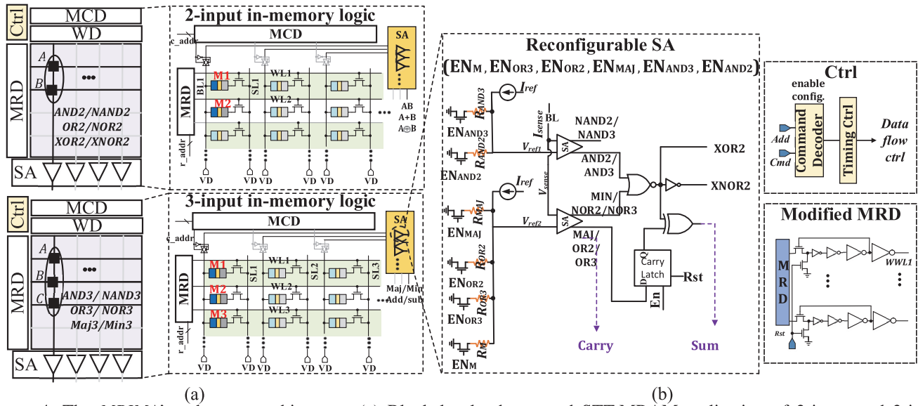
Figure 4: The MRIMA 's sub-array architecture: (a) Block level scheme and STT-MRAM realization of 2-input and 3-input in-memory logic methods, (b) Peripherals of computational sub-arrays to support computation.
