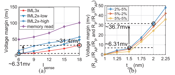
Figure 7: (a) Voltage margin between sensitive states of MRIMA 's operations vs. I_{sense} with a t_{ox}=1.5nm , (b) Voltage margin of IML3x operation vs. thickness of MTJ oxide with different variations on RA_P/TMR with a I_{sense} = 6.6\mu A .
