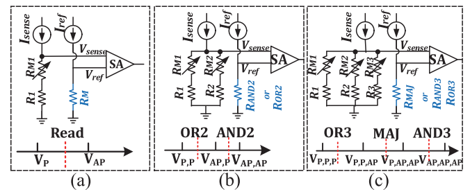
Figure 5: The idea of voltage comparison between V_{sense} and V_{ref} for (a) memory read, (b) IML2x, and (c) IML3x.
