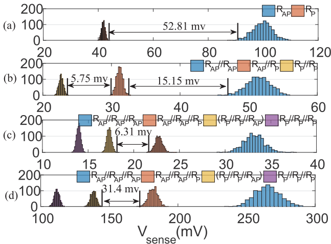
Figure 6: Monte-Carlo simulation of V_{sense} (with RA_P/TMR=2\%/5\% - t_{ox}=1.5nm ) for (a) memory read, (b) IML2x, (c) IML3x when I_{sense} = 6.6\mu A , and (d) IML3x when I_{sense} = 18\mu A .
