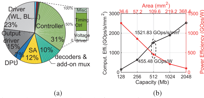
Figure 12: (a) Area overhead of MRIMA in a memory group, (b) Area-peak performance trade-off.
