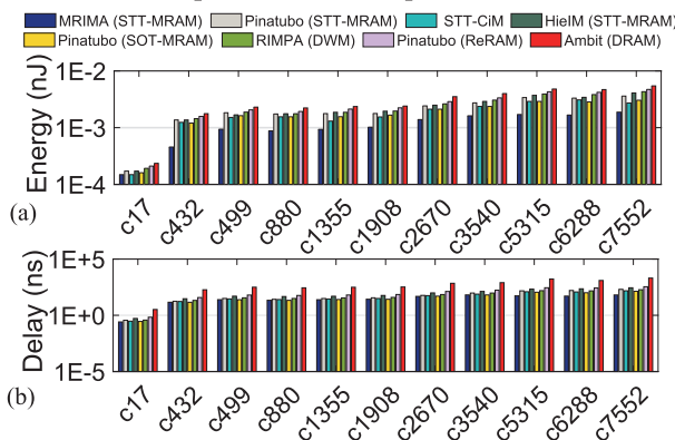
Figure 13: (a) Energy and (b) Delay of ISCAS85 benchmarks (Y-axis: Log scale).
