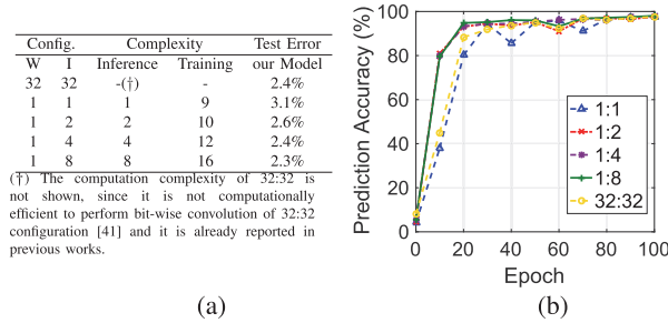
Figure 14: (a) Test error of the CNN model, (b) Prediction accuracy vs. epoch.
