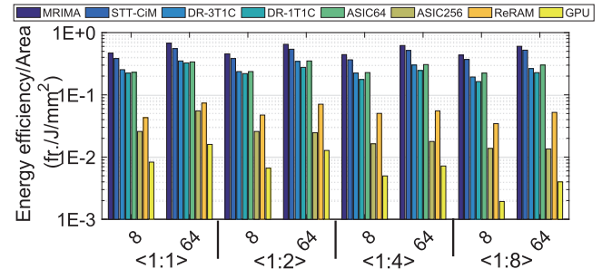
Figure 15: Energy-efficiency of different CNN accelerators.
