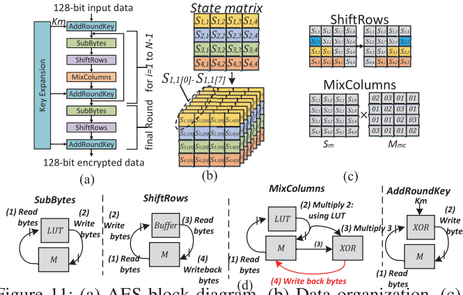
Figure 11: (a) AES block diagram, (b) Data organization, (c) ShiftRows and MixColumns transformation, (d) Mapping of AES's transformations to MRIMA .
