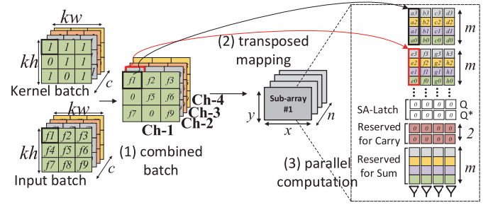
Figure 8: Data organization and computation steps of binary-weight layers.
