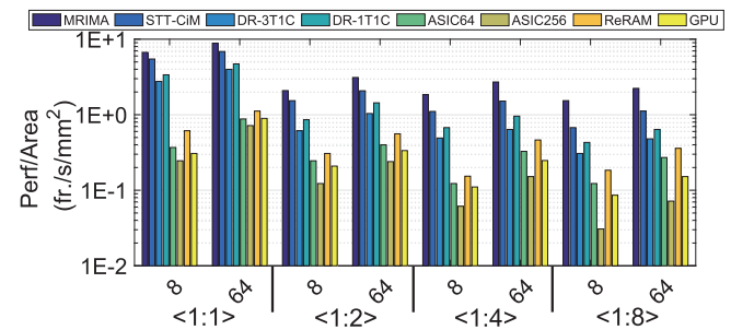
Figure 16: Performance of different CNN accelerators.
