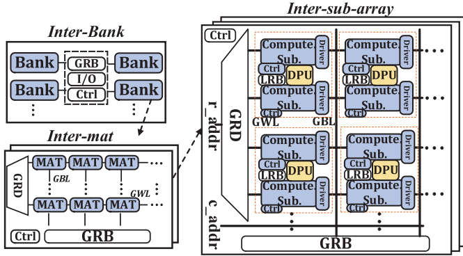
Figure 2: MRIMA architecture.
