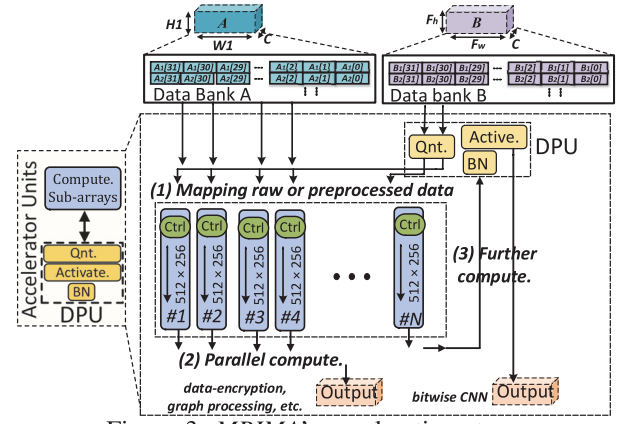
Figure 3: MRIMA's acceleration steps.
