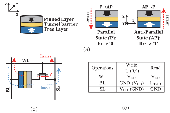
Figure 1: (a) Device structure of MTJ, (b) 1T1R STT-MRAM, (c) Biasing conditions.
