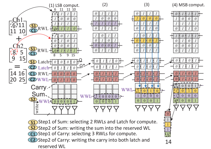
Figure 9: Parallel in-memory addition steps for generating sum and carry-out logic.
