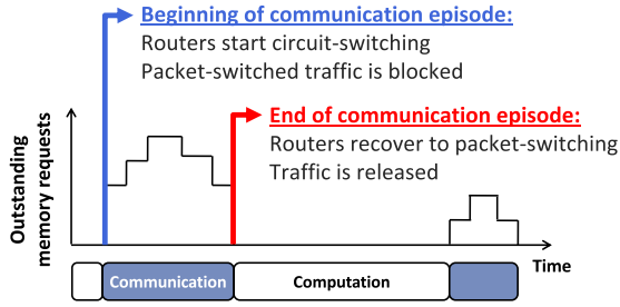
Fig. 3. Hybrid NoC with predictive reservation.
