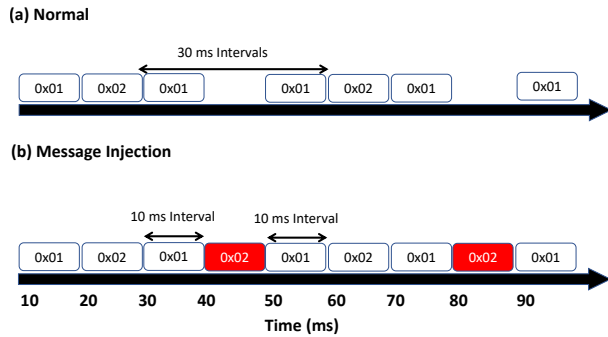
Fig. 2. Transmitted messages on CAN bus (a) under normal status and (b) under message injection attack. The time interval of message CAN ID 0x02 is shortened by the injection of attack messages. Based on Song et al. [15]
