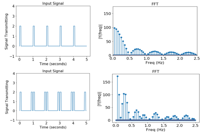
Figure 7: As the message rate doubles during injection attack, the magnitudes of certain frequency peaks will increase.
