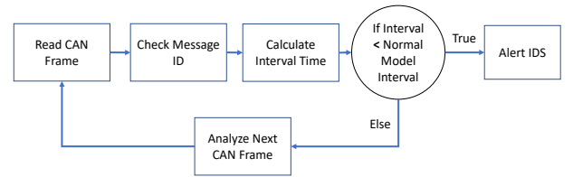
Figure 2: Every CAN message is read and its ID captured. The time interval from current to previous message with the same ID is calculated and compared to the normal model timing interval for that message. If the interval time is less than normal, the IDS will indicate an anomaly and the IDS sends an alert.
