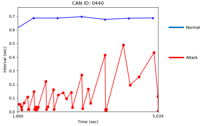
Figure 3: Demonstrating message injection attacks affecting the timings of messages. The simulated attack messages have fluctuating message timings and are shorter than normal depending on rate of injection.
