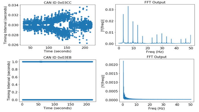
Figure 6: On the left side there are two examples of CAN messages with irregular timing intervals. The right side shows their respective FFT outputs. Variations in the message timings can affect the FFT output.
