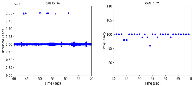
Figure 8: CAN message 0x7A varied when the vehicle shifted driving modes. The timing interval increased by a factor of 2. However, the message frequency of the same message over the same driving transitions, the frequency does not vary more than 5 percent.
