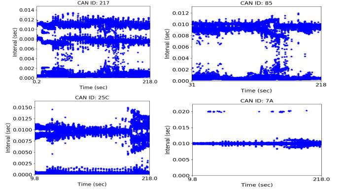
Figure 4: Multiple CAN messages show varying message intervals. Some messages show multiple distinct intervals while some vary due to changes in vehicle operations.
