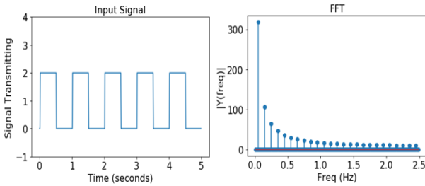
Figure 5: Left plot depicts an ideal square wave, which represents the converted CAN message data. The messages get transmitted at a fixed interval and have a certain transmission time represented by the duty cycle of the wave. The right plot shows the Fourier transform of the square wave.
