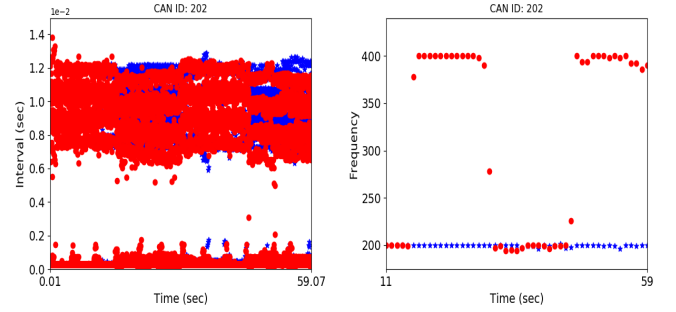
Figure 9: A comparison of the effect message injection attack has on the interval and frequency of CAN ID: 0x202. Left: Message shows multiple variable timing intervals. Injection attack (red) alters the interval of messages by shortening them. Right: By changing timing to frequency, it is clear when message injection attack is occurring, it can be shown that the frequency is consistently at 200 msgs per second normally (blue).
