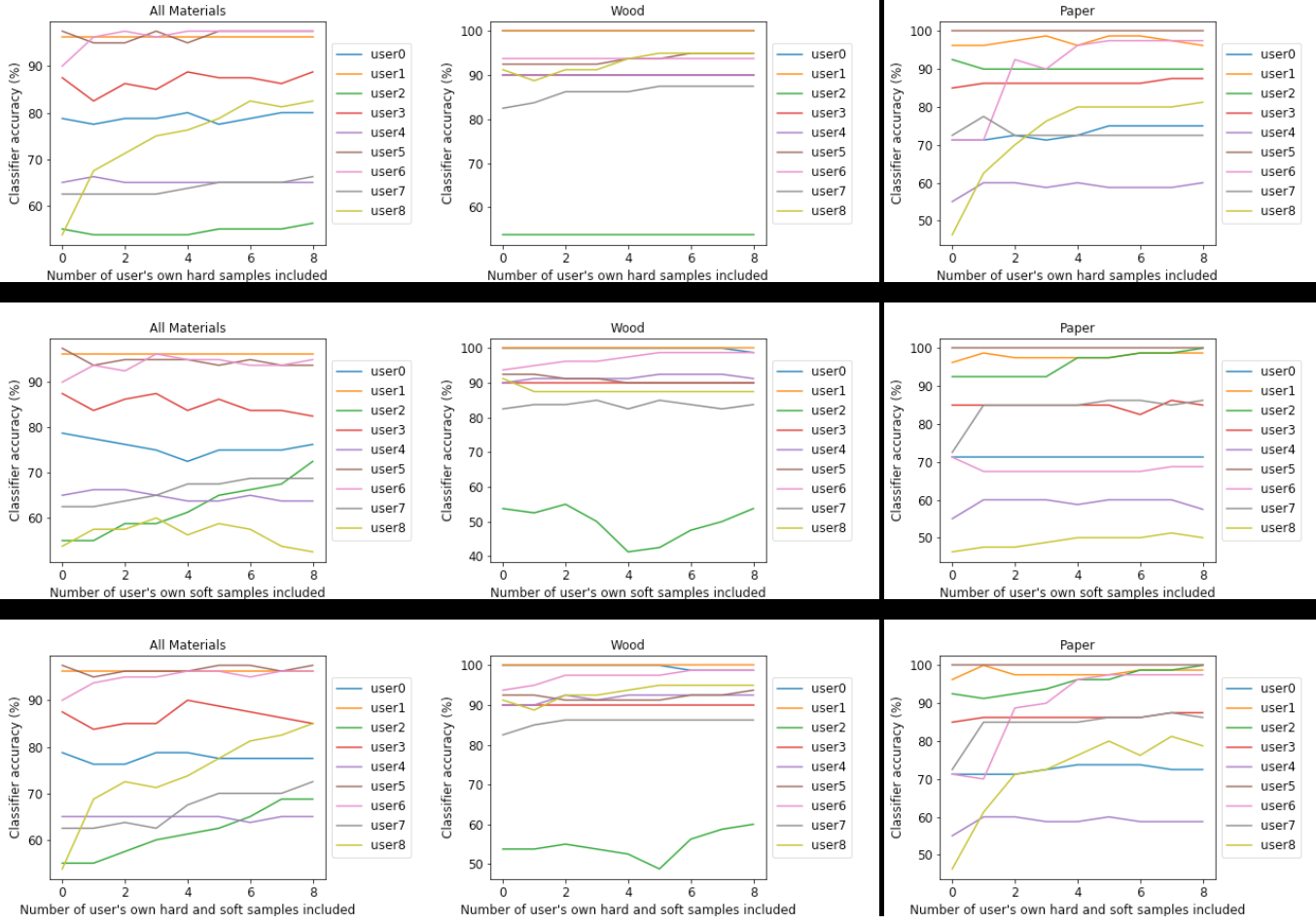
Fig. 4. Change in user-aware classification with addition of increasing numbers of hard swipes only from the user (top), soft swipes only from the user (middle), and hard and soft swipes from the user (bottom) for all materials (left), wood (center), and paper (right). The horizontal axis for the bottom row represents the number of hard and number of soft swipes used, e.g., 4 indicates that 4 hard and 4 swipes are used, i.e., a total of 8 swipes. The accuracy at 0 on the horizontal axis represents user-agnostic classification.
