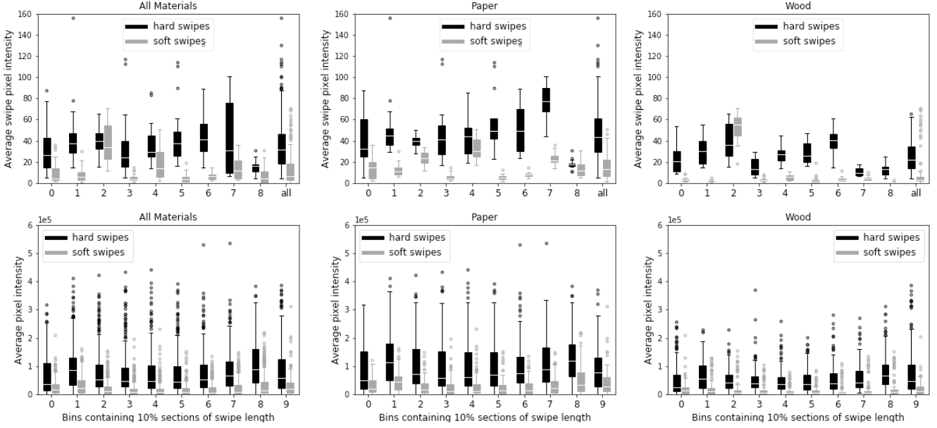
Fig. 2. Box plots for each user of average pixel intensity over a swipe, created using 16 hard and 16 soft swipes per user for all materials, paper only, and wood only.
