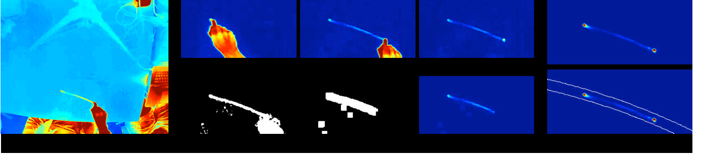
Fig. 1. (a) Thermal intensity image of a user performing a swipe recorded by an overhead FLIR Vue Pro 640 thermal camera. (b) Sample frames from a video of a swipe, showing the start of the swipe (left), end of the swipe (center), and swipe after the user removes the hand (right). (c) Thresholded finger swipe image (left), thresholded image with hand removed using morphological operations (center), and masked finger swipe (right). (d) Accumulative intensity image (top) and quadratic band fit to accumulative image (bottom).
