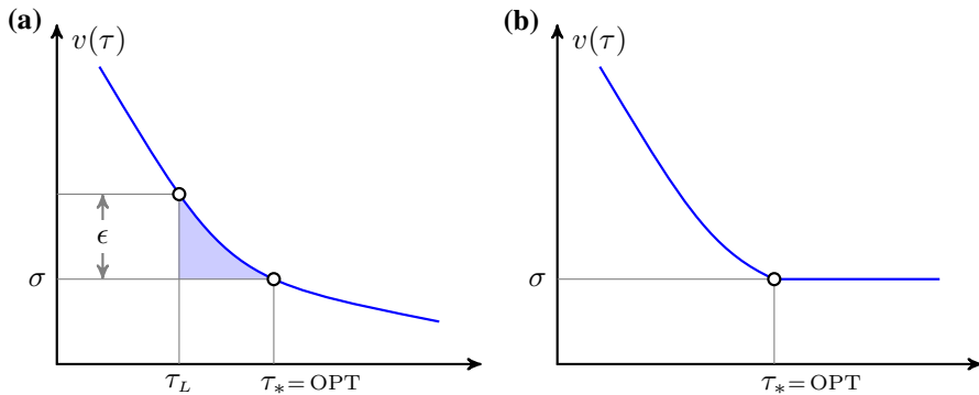
Fig. 1 a The shaded area indicates the set of allowable solutions \tau \in [\tau_L, \tau_*] to the root-finding problem (1.1), and corresponds to the set of super-optimal solutions x that satisfy (1.2); b the root may be a minimizer of v , and then \tau_* corresponds to the left-most root
