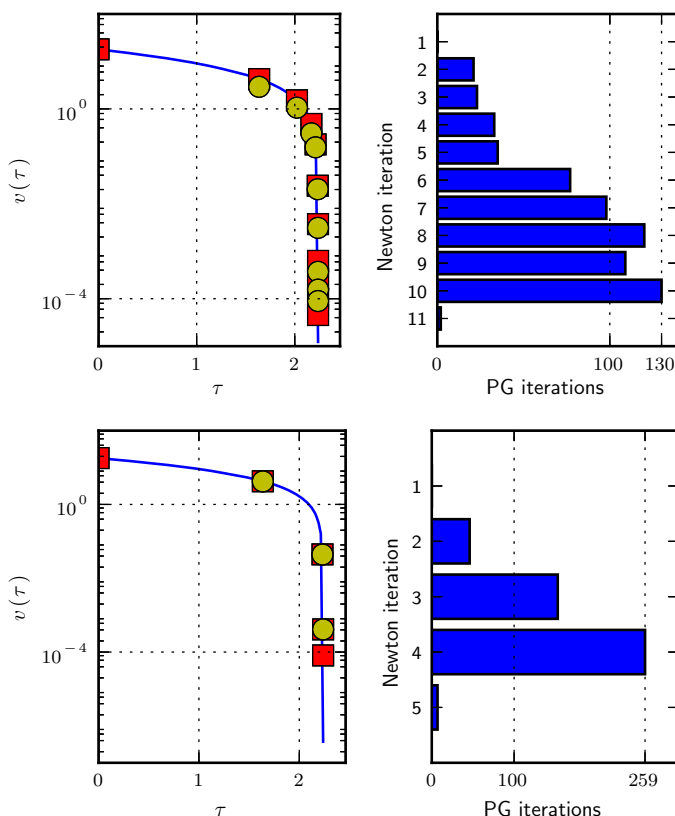
Fig. 3 Progress of the least-squares level-set method for a linear program (cf. Sect. 4.1.1). The panels on the left depict the graph of v(\tau) (solid line), and the squares and circles, respectively, show the upper and lower bounds computed using an optimal projected-gradient method. The horizontal log scale results in a value function that appears nonconvex. The panels on the right show the number of projected-gradient iterations for each Newton step. Top panels: \alpha = 1.8 . Bottom panels: \alpha = 1.01
