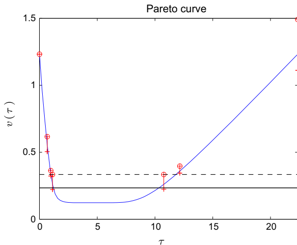
Fig. 4 A plot of the value function v(\tau) of (4.11). Newton’s method converges to either the min- or max-trace solution, depending on initialization. To solve (4.10), we need the maximal root. Here, \sigma = 0.25 , indicated by the solid horizontal line
