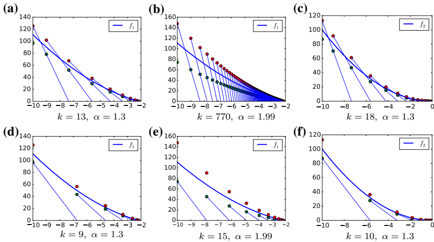
Fig. 2 Inexact secant method (top row) and Newton method (bottom row) for root finding on the functions f_1(\tau) = (\tau - 1)^2 - 10 (first two columns) and f_2(\tau) = \tau^2 (last column). Below each panel, \alpha is the oracle accuracy, and k is the number of iterations needed to converge, i.e., to reach f_i(\tau_k) \leq \epsilon . For all problems, \epsilon = 10^{-2} ; the horizontal axis is \tau , and the vertical axis is f_i(\tau)
