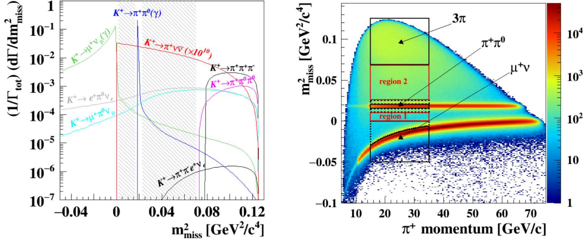
Figure 2: Left: true m^2_{\text{miss}} distribution of the K^+ \rightarrow \pi^+ \nu \bar{\nu} decay and the main K^+ decays, computed under \pi^+ mass hypothesis for the charged particle in the final state. Signal (red) is multiplied by 10^{10} for visibility and the dashed areas show the signal search regions. Right: reconstructed m^2_{\text{miss}} as a function of \pi^+ momentum for control events selected without applying \pi^+ identification and photon rejection. Signal regions 1 and 2, as well as the 3\pi , \pi^+ \pi^0 and \mu^+ \nu background regions are also shown. The control regions located between the signal and background regions are indicated by dashed lines.
