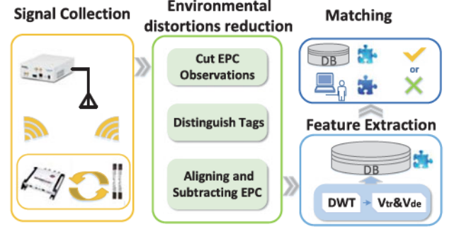
Fig. 6. System workflow.
