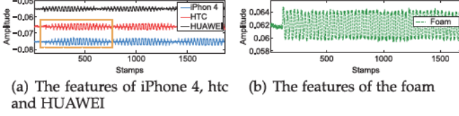
Fig. 17. Feature C_a of different types of items after DWT.
