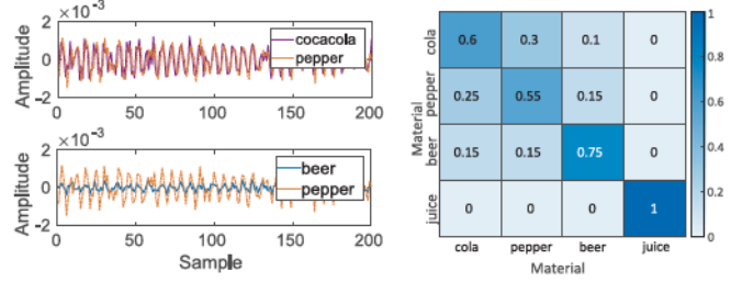
(a) The features of different drinks
