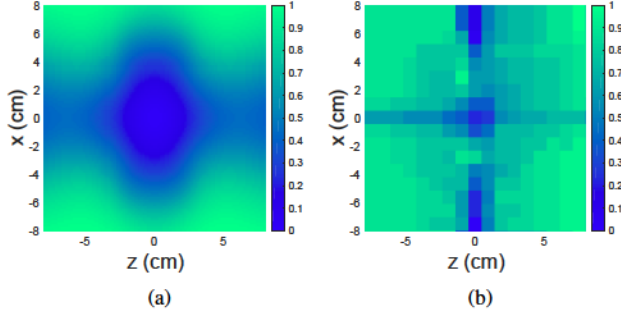
Fig. 9. RSS distribution with one reference pair locating at different positions in the x - z plane. (a) simulation results derived from the theoretical model (b) RSS collected from real measurements.
