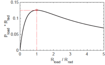
Fig. 4. The relationship between the obtained IC power and the ratio of the load to radiation resistance.
