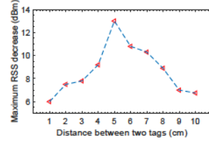
Fig. 14. Impact of interval within reference pair.
