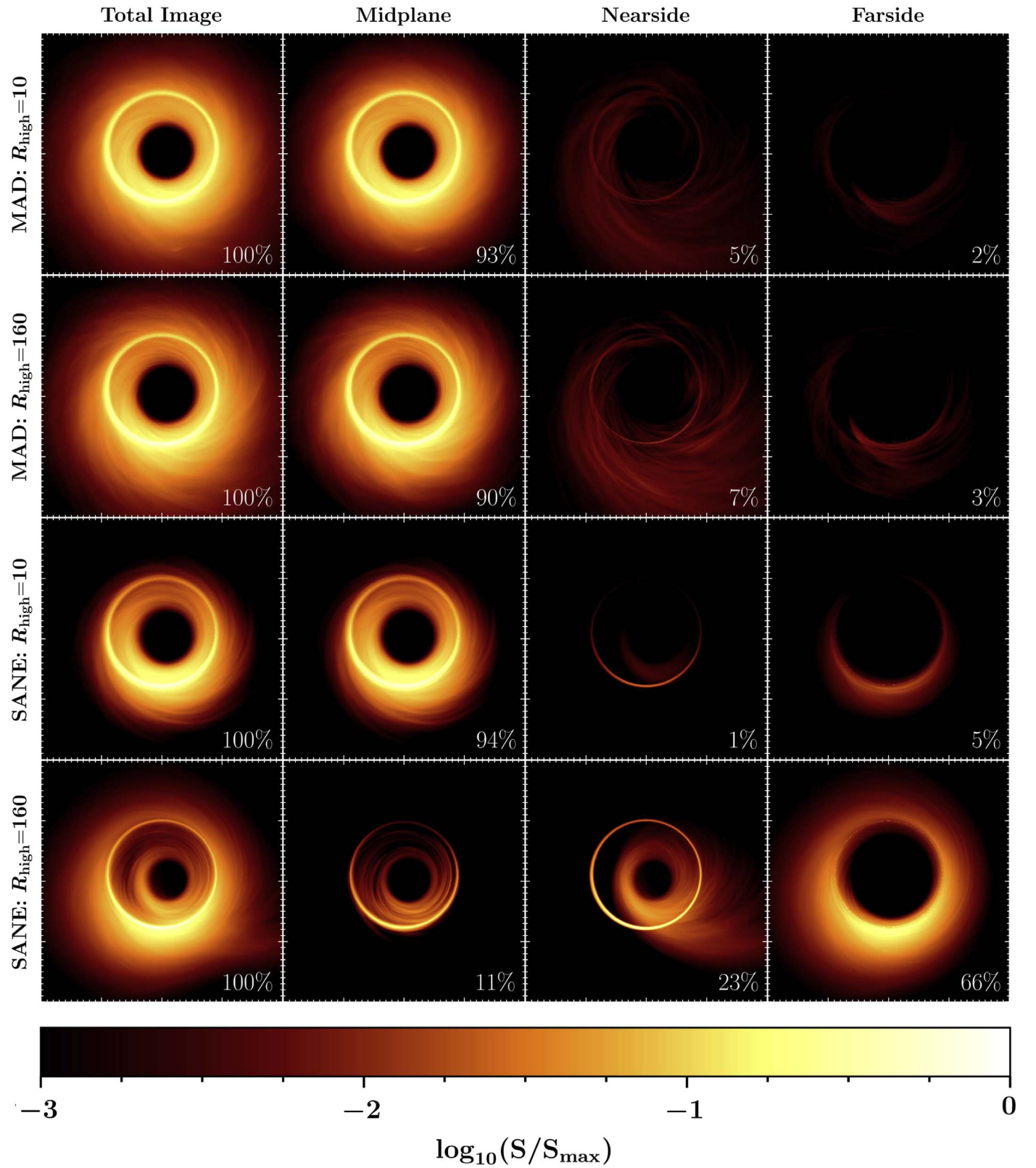
Figure 11. Decomposition of time-averaged 1.3 mm images from Figure 4 into midplane, nearside, and farside components (MAD and SANE models with a_* = 0.94 ). Each model (row) of the figure corresponds to a simulation in Figure 4. The percentage of the total image flux from each component is indicated in the bottom right of each panel. The color scale is logarithmic and spans three decades in total flux with respect to the total image from each model, chosen in order to emphasize both nearside and farside components, which are nearly invisible when shown in a linear scale. The field of view is 80 \mu\text{s} .
