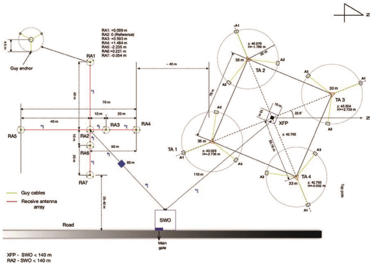
Figure 2. Configuration of JBS-VIPER antenna arrays. The radiating part in transmitting (Tx) towers consists of wire longer than 1.5 km length in 4 zig-zag planes. Seven receive antennas are cruciformly located beside four Tx towers.
