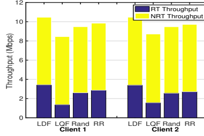
Figure 7: Throughputs for K_{RT}=3 and K_{NRT}=6 .
