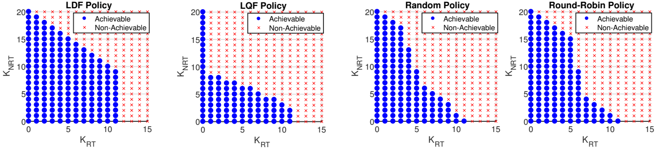
Figure 5: Capacity Regions for the different Policies with 5 ms deadline and 0.99 delivery ratio.
