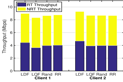
Figure 6: Throughputs for K_{RT}=4 and K_{NRT}=4 .
