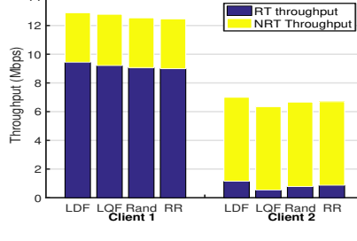
Figure 10: Throughputs for the arrival process with P(K_{RT1}) = 0.8 , P(K_{NRT1}) = 0.3 , P(K_{RT2}) = 0.1 , P(K_{NRT2}) = 0.5 .
