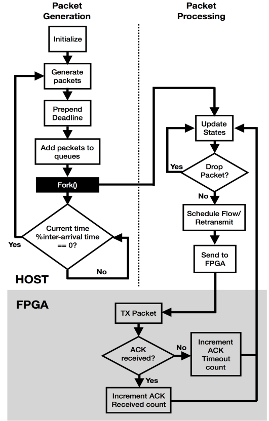
Figure 1: Architecture of PULS. Packet generation and Packet Processing happen at the host simultaneously (indicated by “Fork”), while low-level functionalities occur at the hardware (FPGA) level.
