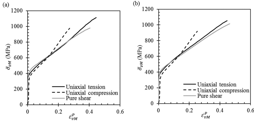
Fig. 2. Von Mises equivalent stress, \bar{\sigma}_{vM} , versus von Mises equivalent plastic strain, \bar{\epsilon}_{vM}^P , for representative tests on samples extracted from the (a) 80% SS304L wall, and (b) 90% SS304L wall.
