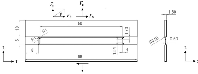
Fig. 1. Geometry of a multiaxial plasticity specimen (units: mm), with the orientations of the vertical force, F_v , and horizontal force, F_h , along with the biaxial loading angle, \beta , drawn. Sample geometry adapted from [62]. L is the longitudinal direction, parallel to the length of the wall, T is the vertical build direction, and z is the wall thickness direction.
