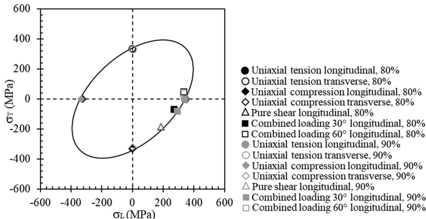
Fig. 3. Engineering yield stress in the transverse direction, \sigma_T , versus engineering yield stress in the longitudinal direction, \sigma_L , for plane stress, in the 80% and 90% SS304L walls as measured by experiments (symbols). The fitted von Mises yield surface, based on uniaxial tension in the longitudinal direction, is shown as a solid line.
