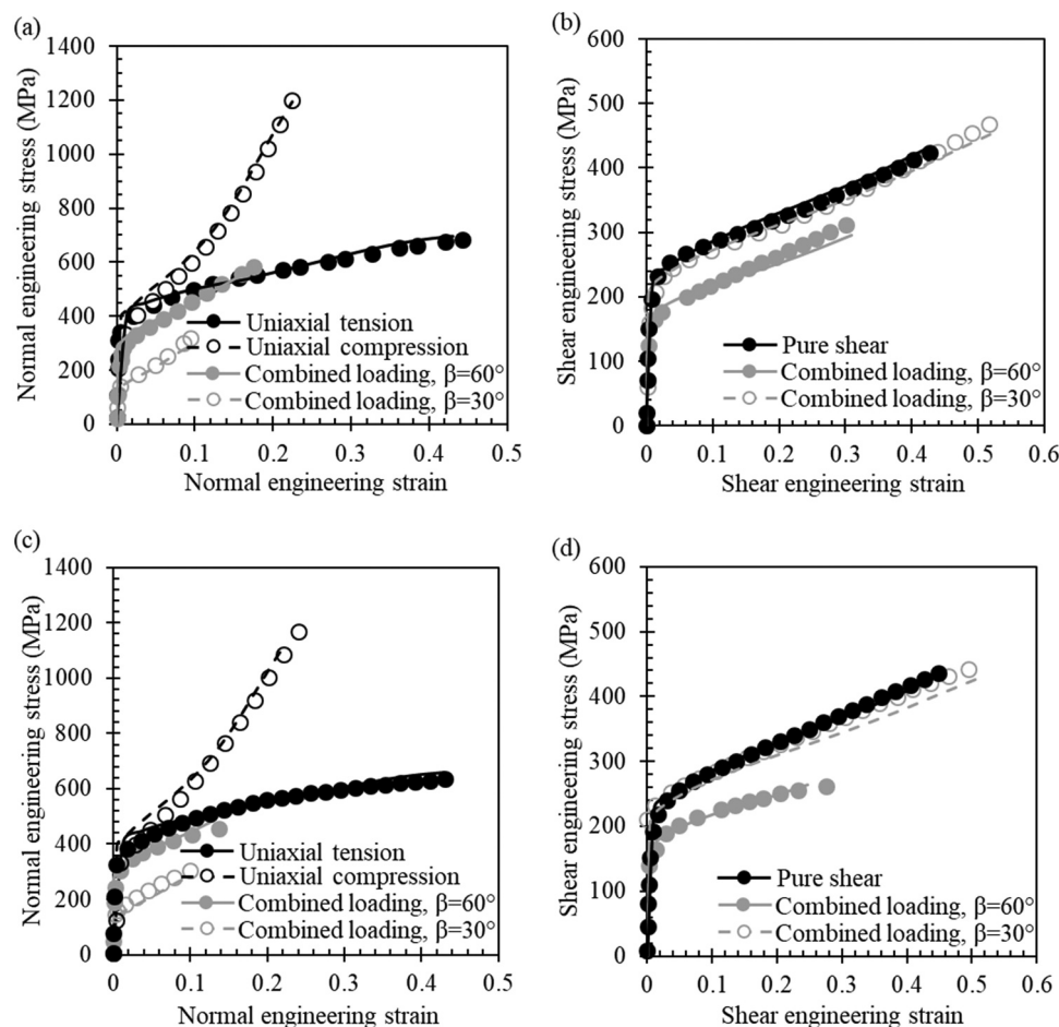
Fig. 4. Normal engineering stress-strain curves for specimens under uniaxial tension, uniaxial compression, and combined loading for the (a) 80% SS304L wall and (c) 90% wall. Shear engineering stress-strain curves for specimens under pure shear and combined loading for the (b) 80% SS304L wall and (d) 90% SS304L wall. Symbols correspond to experimental results and lines correspond to results predicted by the calibrated plasticity model. Curves obtained under uniaxial tension, uniaxial compression, and pure shear were used for model calibration and curves under combined loading were used for model validation.
