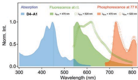
Fig. 5 Normalized absorption and emission spectra of D4-A1 in 1:1 EtOH : DCM.
