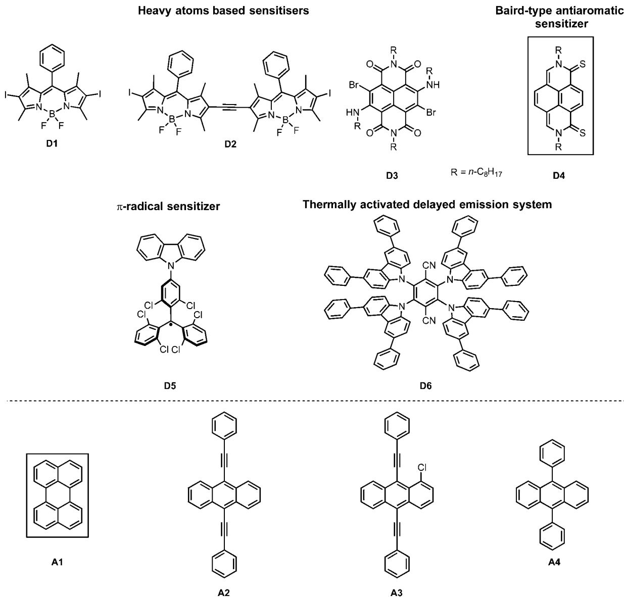
Fig. 1 Molecular structures of model organic triplet sensitizers D1–D5 and corresponding triplet energy PAH acceptors A1–A4 , which have successfully used for TTA-PUC. Due to their structural similarity, we believe that D4 and A1 are compatible structures that can be tailored for single component TTA-PUC research. 20
