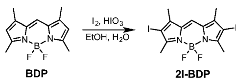
Scheme 1 Synthesis of heavy atom containing BODIPY dyes reported by Nagano and co-workers. 40
