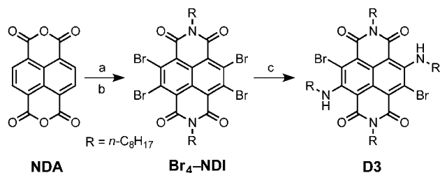
Scheme 2 Synthesis of photosensitizer D3 : (a) dibromoisocyanuric acid, oleum (20% \text{SO}_3 ), 25 °C, 3 h; (b) n -octylamine, acetic acid, 90 °C, 30 min, \text{N}_2 , then \text{PBr}_3 , dry toluene, reflux, 12 h; (c) n -octylamine, dry dimethylformamide, 135 °C, 6 h. 27
