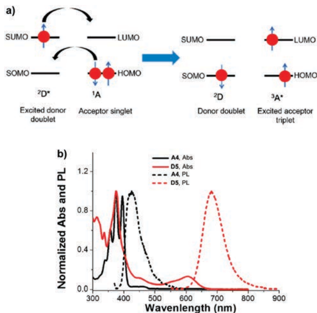
Fig. 7 (a) Schematic representation of Dexter-like doublet-triplet energy transfer. (b) Normalized absorption and emission spectra of D5 (0.1 mM; \lambda_{\text{Exc}} = 530 nm) and A4 (0.1 mM; \lambda_{\text{Exc}} = 375 nm) in toluene. Adapted with permission from ref. 36. Copyright 2017 American Chemical Society.
