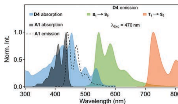
Fig. 2 Normalized absorption and emission spectra of D4 and A1 in 1:1 EtOH : DCM. The phosphorescence ( \text{T}_1 \rightarrow \text{S}_0 ) of D4 was recorded 100 \mu\text{s} after pulsed excitation in EtOH:DCM glass at 77 K. Adapted with permission from ref. 30. Copyright 2017 American Chemical Society.
