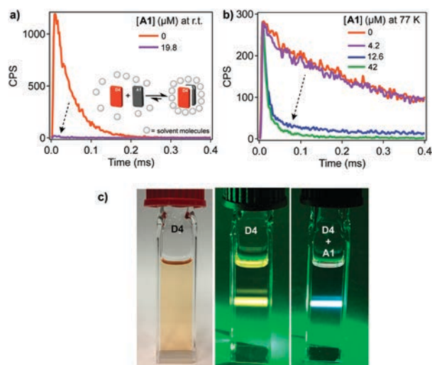
Fig. 3 Phosphorescence (monitored at 725 \text{ nm} ) decay traces of D4 (conc. = 1.71 \times 10^{-5} \text{ M} ) in the presence of A1 at (a) room temperature in deaerated 1 : 1 EtOH : DCM (inset: graphical illustration of intermolecular or bi-molecular interaction of D4 and A1 in solution or condensed matrices) and (b) at 77 \text{ K} in 1 : 1 EtOH : DCM glassy matrix. (c) Photograph of photoluminescence of D4 (left) and A1 upconverted photoluminescence in deaerated THF (right) using a 532 \text{ nm} commercial laser ( 30\text{--}40 \text{ mW cm}^{-2} ). Adapted with permission from ref. 30. Copyright 2017 American Chemical Society.
