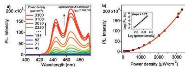
Fig. 4 (a) Intensity-dependent upconverted emission of A1 in the presence of D4 excited at 532 \text{ nm} ( [\text{D4}] = 7.04 \times 10^{-5} \text{ M} ; [\text{A1}] = 21.12 \times 10^{-5} \text{ M} ) in deaerated THF; a 500 \text{ nm} shortpass filter was used to discard the overlapping emission from D4 as well as cutting off the incident radiation. (b) Best quadratic fit ( \chi^2 ) of the PL intensity at 465 \text{ nm} . Inset: Double logarithmic plot PL intensity vs. power density of the incident light producing a linear fit with slope = 1.75 . Adapted with permission from ref. 30. Copyright 2017 American Chemical Society.
