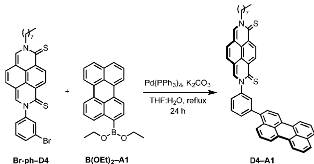
Scheme 4 Synthesis of dyad D4-A1 via Suzuki coupling. The detailed synthesis of starting materials Br-ph-D4 and B(OEt) 2 -A1 can be retrieved in the ESI†
