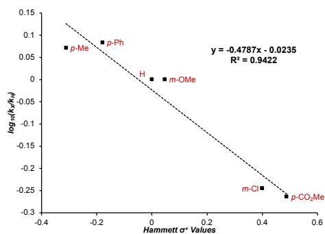
Figure 1. Plot of \log(k_X/k_H) versus Hammett \sigma^+ values derived from the scope presented in Scheme 3 and see also SI.
