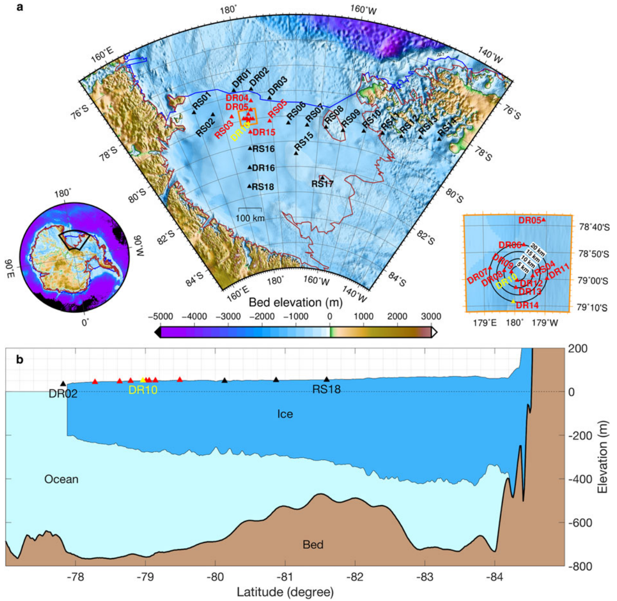
Fig. 1. (a) The RIS seismic stations (triangles) superimposed on the bed elevation map (Fretwell and others, 2013), with the center station DR10 (yellow), extended center subarray (red) and other stations (black) indicated. The RIS is bounded by the grounding line (brown line) and the ice front (blue line). An expanded view of the dense center subarray (orange box) is shown in the right inset, where the contours of distance to DR10 are shown (black circles). (b) Cross-section along the 180° meridian (Fretwell and others, 2013). DR02 is off the ice front because the ice front has moved northward, but the ice thickness model has not been updated.
