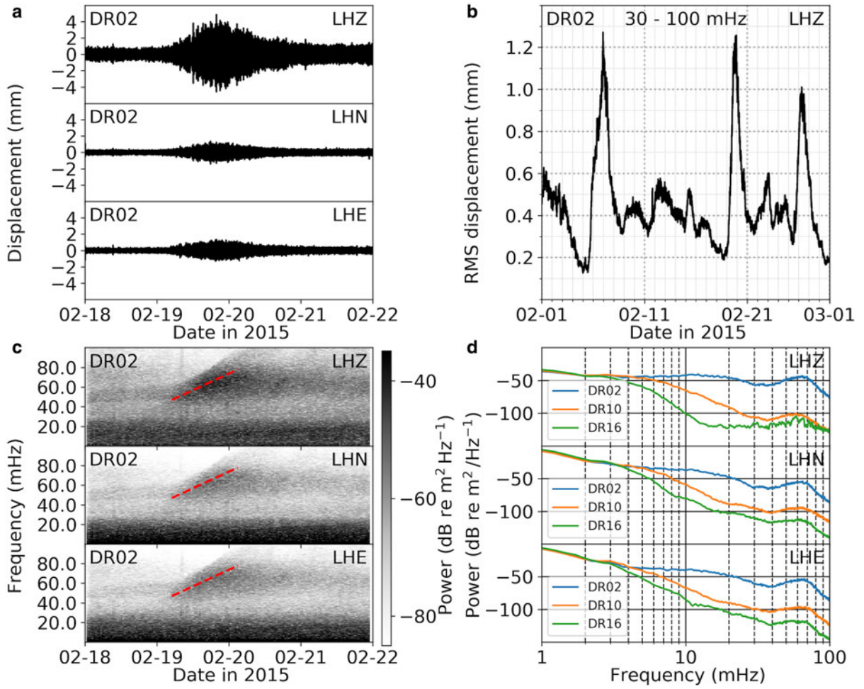
Fig. 6. RIS response to a swell event from 02:00 on 19 February to 10:00 on 21 February, 2015: (a) 4-day seismograms at DR02 (bandpassed 30–100 mHz). (b) RMS of the vertical displacements at DR02 (bandpassed 30–100 mHz) in February 2015. RMS window length is 4096 s. (c) Displacement spectrogram at DR02. The dispersion trend slope (red dashed) indicates a source distance of \sim 2000 km. (d) Displacement spectrum at DR02 (blue), DR10 (orange) and DR16 (green) from 19 February 02:00 to 21 February 10:00. The vertical LHZ and horizontal LHN and LHE components are indicated in each subplot.
