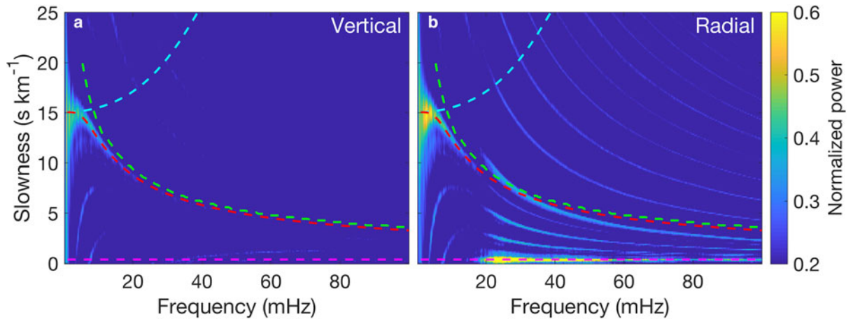
Fig. 8. RIS response to a swell event from 02:00 on 19 February to 10:00 on 21 February, 2015: Dispersion curves of (a) vertical and (b) radial components, obtained by averaging the beamforming output over 0^\circ to 20^\circ azimuth (the north-south line subarray is roughly along 10^\circ ). Phase speed dispersion curves of ocean surface gravity waves (cyan), flexural waves (green), flexural-gravity waves (red) and S_0^* (magenta) in the AIWB model (see Fig. 3) are overlaid for comparison. The subplots are normalized to the maximum value over the two subplots.
