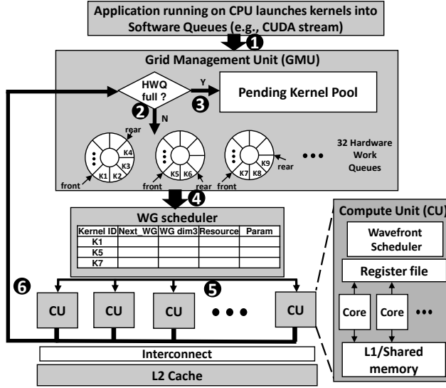
Fig. 2. Baseline GPU architecture.
