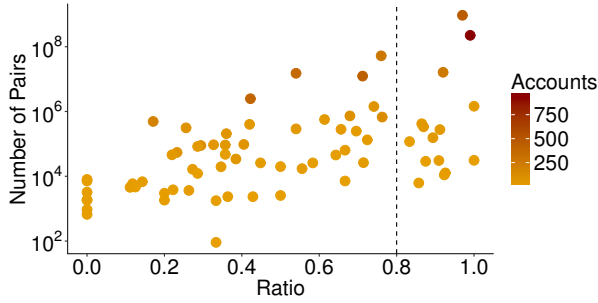
Figure 8: Scatterplot for 71 fraudster communities (shown as dots) discovered by PFD: the percentage of users who wrote reviews that are at least 50% Jaccard similar to other reviews ( x axis) vs. the number of review pairs (in log scale) in each component ( y axis). 15 communities have at least 80% of their user accounts suspected of plagiarism.
