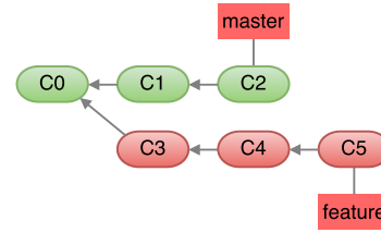
Figure 3: A regular commit on the feature branch.
