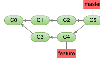
Figure 4: Merge commit from merging two branches.
