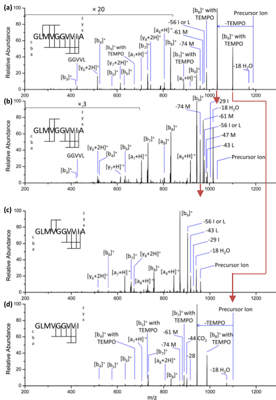
Figure 4. The MS 2 on singly protonated CL-FRIPS-derivatized \beta -amyloid peptide (33–42) (a), MS 3 on the ion representing the loss of TEMPO (b), MS 3 on –74 side chain loss ion (c), and MS 2 on [b 9 ] + with TEMPO ion (d)
