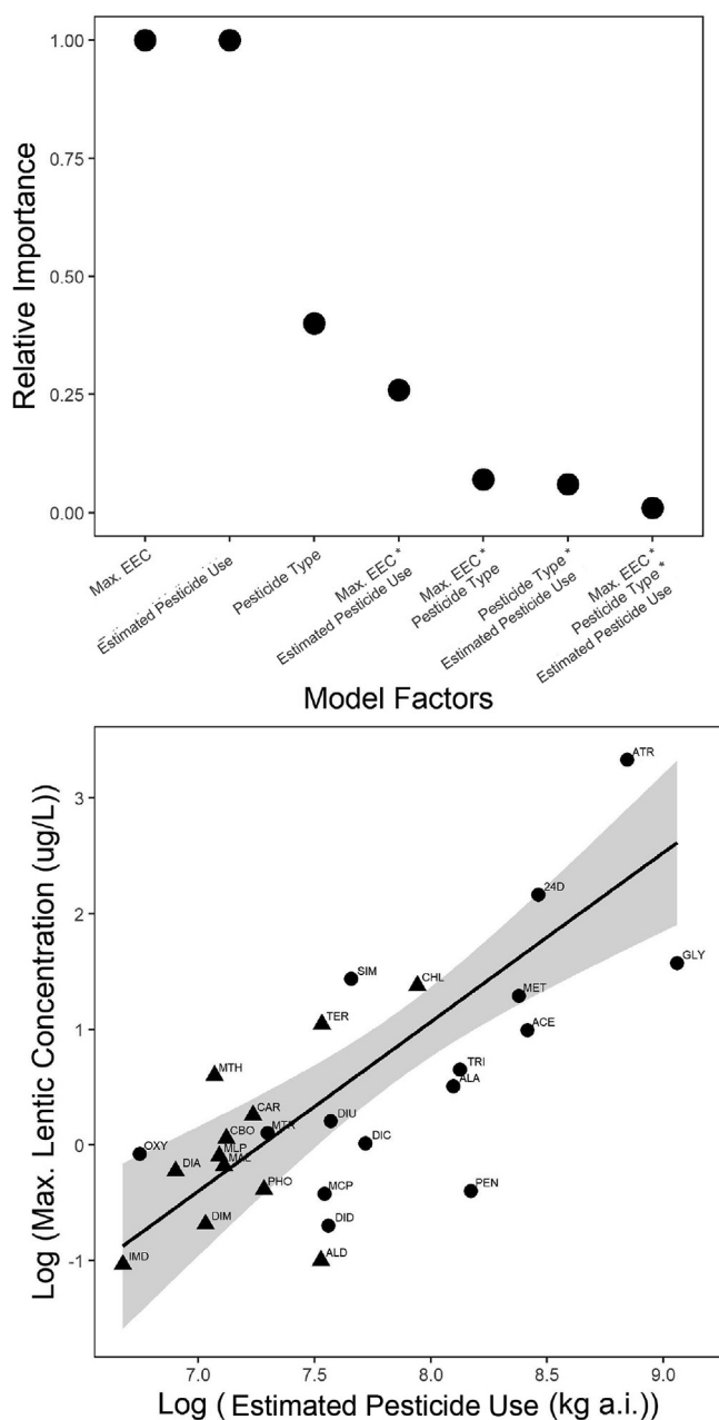
Fig. 3. A) Relative importance scores of factors from model comparisons, evaluating the best predictors of maximum concentration of pesticides in lentic systems. Maximum estimated environmental concentration is abbreviated as Max. EEC. B) Conditional plot displaying the significant effect of estimated pesticide use on maximum (max.) lentic concentration, controlling for maximum EEC, soil half-life, and pesticide type (based on best fitting model, Table 2, F = 30.594 , p < 0.001 ). Gray bands represent 95% confidence intervals. Conditional plot was generated using the visreg package in R.
