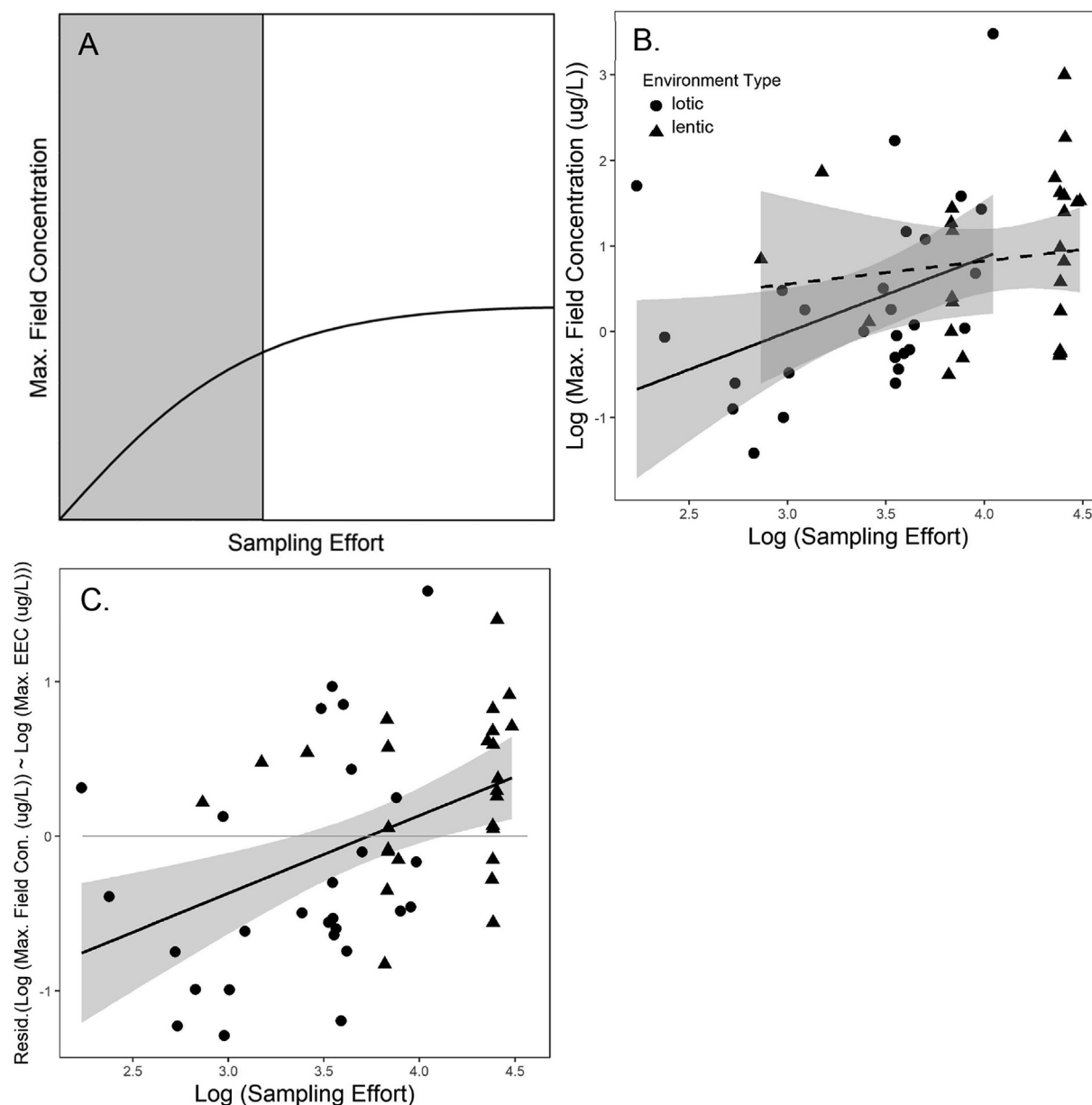
Fig. 1. A) Predicted asymptotic relationship between sampling effort and maximum (max.) field concentration. As sampling effort increases, the likelihood of detecting a peak concentration increases when sampling effort is at low to mid-levels as shown in gray. At mid to high levels of sampling effort, the influence of increased sampling effort on the likelihood of detecting a peak concentration reaches a limit, and no discernible relationship exists between sampling effort and max. field concentration as shown in white. We predict that sampling effort would account for more variance between maximum field concentration and maximum estimated environmental concentration (EEC) when sampling effort occurs in the lower range (in gray) compared to the higher range (in white). B) Observed relationship between sampling effort and maximum field concentration in lotic (circles, solid line) and lentic (triangles, dashed line) systems. Increased sampling effort is positively associated with maximum lentic concentration (Table 2, F = 4.552 , p = 0.043 ) but not maximum lotic concentration (Table 2, F = 0.436 , p = 0.515 ). The positive relationship for lentic systems matches the positive relationship at low to mid-sampling effort shown in gray in Fig. 1B. The absence of a relationship for lotic systems matches the asymptote at mid to high sampling effort in Fig. 1B. C) Observed relationship between sampling effort and the residuals of maximum field concentrations in lotic (circles) and lentic (triangles) in systems and EEC (Table 2, \chi^2 = 12.339 , p < 0.001 ). As sampling effort increases, the likelihood of a field concentration exceeding an EEC increases, which is represented by a positive residual. Gray band represent a 95% confidence interval, and a light gray reference line at 0 represents where maximum field concentration would equal maximum EEC.
