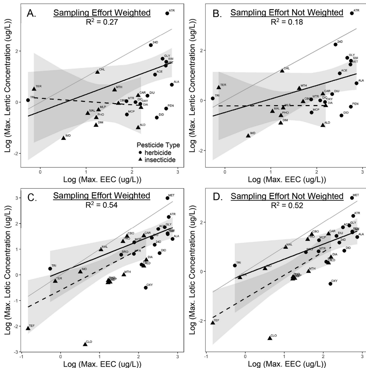
Fig. 2. Associations between herbicide and insecticide maximum (max.) estimated environmental concentrations (EEC) and measured maximum field concentrations in lentic (A and B) and lotic (C and D) systems. Models were built with (A and C) and without (B and D) observations weighted by sampling effort. The association between maximum EEC and maximum field concentration is significant for the lotic system with and without observations weighted by sampling effort (Table 2, p < 0.001 , C and D) and nearly significant for lentic system when observations are weighted by sampling effort (Table 2, p = 0.052 , A and B). In all panels herbicides are shown with solid circles and solid lines, and insecticides are shown with triangles and dashed lines. Individual pesticides are shown above and to the left of the point (see Table 1 for abbreviations). Gray bands represent 95% confidence intervals, and light gray lines are 1:1 reference lines.
