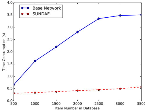
Figure 9: Extensibility comparison between SUND AE and alternative architecture.
