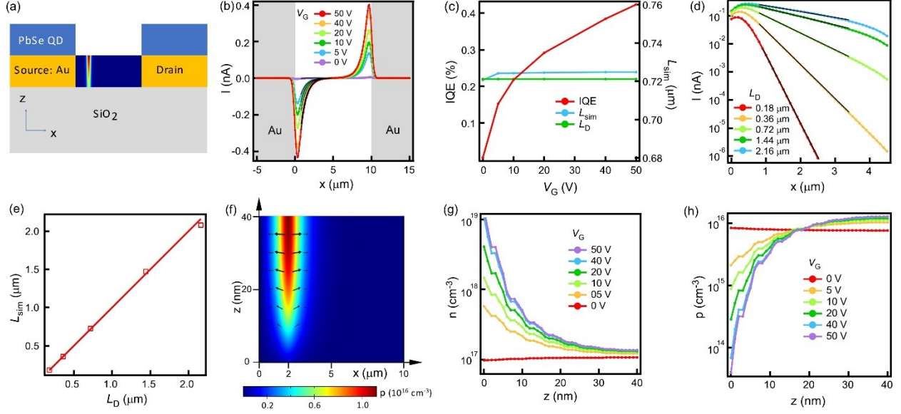
Figure 2. Simulated photocurrent distribution in a PbSe QD FET with local photoexcitation. All simulations are performed at V_{SD} = 0 V. (a) Schematic of a typical device illuminated by a focused laser beam. The color map between source and drain represents the distribution of carrier generation as the laser is centered at x = 2 \mu\text{m} . (b) Photocurrent as a function of photoexcitation position at various V_G , with I_{\text{ex}} = 0.8 \text{W}/\text{cm}^2 and L_D = 0.72 \mu\text{m} . The shaded areas indicate the Au contacts. The black curves are exponential fittings. (c) IQE at the maximum photocurrent position and L_{\text{sim}} extracted from (b) as a function of V_G . (d) Semi-log plots of photocurrent vs. photoexcitation position with different L_D . The black curves are exponential fittings. (e) L_{\text{sim}} extracted from (d) vs. L_D . The squares are simulated values and the line is the fitting. (f) Hole concentration map in the channel at V_G = 10 V. The arrows represent the hole current density vector \mathbf{J}_p . (g, h) Vertical distribution of electron and hole concentration at the laser injection point ( x = 2 \mu\text{m} ) for different V_G .
