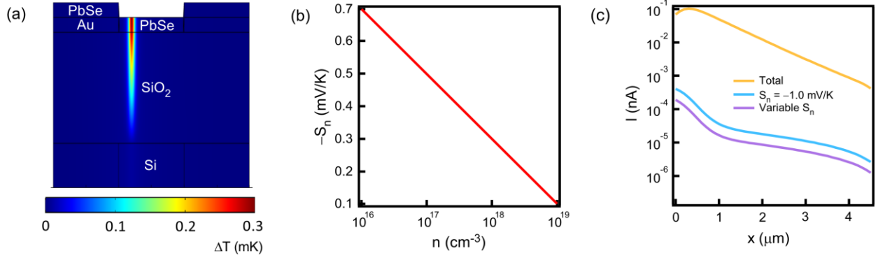
Figure 6. Photo-heating induced thermoelectric effects. (a) Simulated temperature distribution with I_{\text{ex}} = 0.8 \text{ W/cm}^2 at x = 2 \text{ } \mu\text{m} . Dimensions are as shown in Figure 1a. (b) Seebeck coefficient as a function of n calculated from eq 6. (c) Simulated distributions of the total photocurrent and the thermoelectric component at V_{\text{SD}} = 0 \text{ V} , V_{\text{G}} = 10 \text{ V} , and I_{\text{ex}} = 0.8 \text{ W/cm}^2 . Two types of Seebeck coefficients are considered: S_n = -1.0 \text{ mV/K} and n -dependent S_n as in (b).
