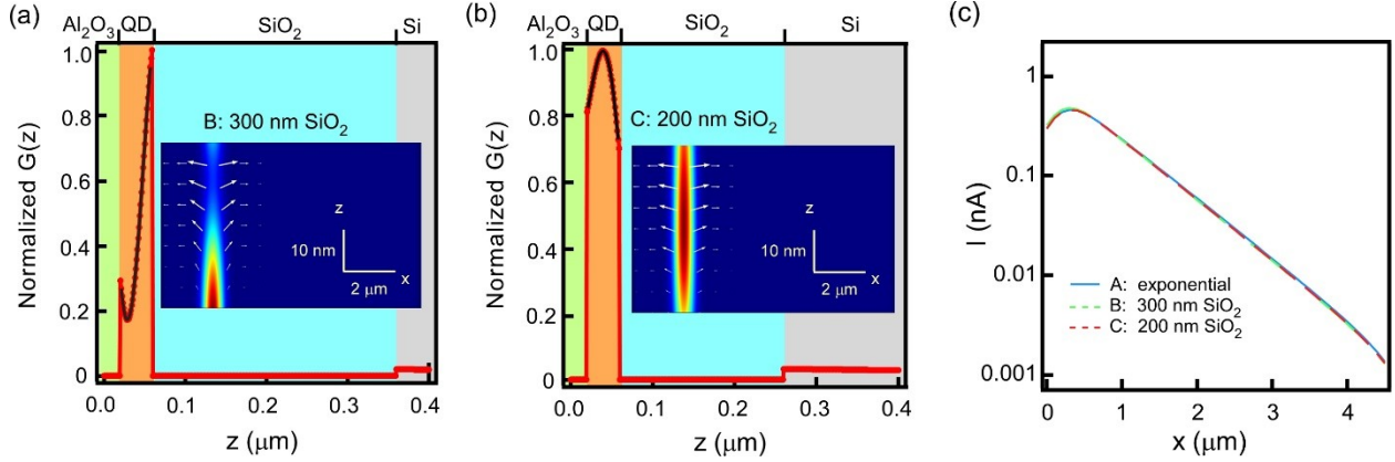
Figure 4. Thin-film optical interference effects. (a, b) The distribution of normalized generation rate with 300 nm and 200 nm \text{SiO}_2 , respectively at photoexcitation wavelength \lambda = 532 nm. The black curves are polynomial fittings. Insets (not in scale, 90 degree rotated from the background Figure 4a,b): 2D profiles of generation in the channel. The arrows represent \mathbf{J}_p . All simulations are performed at V_{\text{SD}} = 0 V. (c) Simulated photocurrent as a function of photoexcitation position with optical interference included. Three types of carrier generation distributions are considered: A, exponential decay, B, interference pattern with 300 nm \text{SiO}_2 , C: interference pattern with 200 nm \text{SiO}_2 . The three curves match perfectly.
