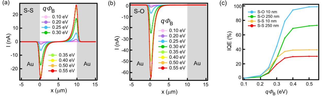
Figure 7. Quantum efficiency as a function of Schottky barrier height q\Phi_B at V_{SD} = 0 \text{ V} . (a, b) Simulated photocurrent profiles at different q\Phi_B with I_{ex} = 0.8 \text{ W/cm}^2 and V_G = 10 \text{ V} for Schottky-Schottky (S-S) and Schottky-Ohmic (S-O) devices, respectively. (c) IQE as function of q\Phi_B for S-S and S-O devices with different beam width \sigma .
