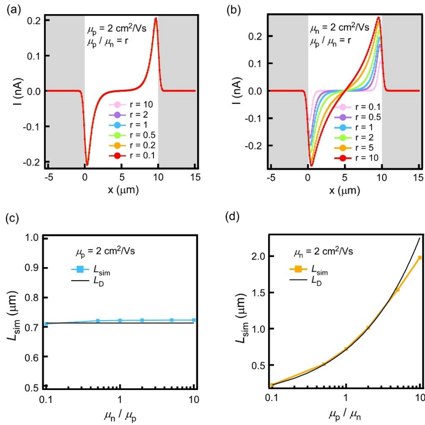
Figure 3. Simulated photocurrent distribution with mismatching electron/hole mobilities. Simulations are performed at V_{\text{SD}} = 0 \text{ V} , V_{\text{G}} = 10 \text{ V} and I_{\text{ex}} = 0.8 \text{ W}/\text{cm}^2 . (a, b) Simulated photocurrent as a function of the electron/hole mobility ratio. The simulations are performed with fixed carrier lifetime ( \tau_n = \tau_p = 100 \text{ ns} ). The ratio r = 0.1 - 10 corresponds to \mu_p/\mu_n . (c, d) L_{\text{sim}} extracted from (a, b), comparing with the calculated L_D .
