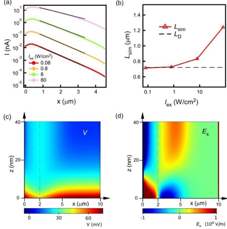
Figure 5. Simulated photocurrent distributions with high-intensity photoexcitation at V_{\text{SD}} = 0 V. (a) Photocurrent as a function of photoexcitation position with different laser intensity, V_G = 10 V, and L_D = 0.72 \mu\text{m} . (b) Fitted decay length L_{\text{sim}} in comparison to L_D for different laser intensities. (c, d) Simulated distributions of V and E_x at I_{\text{ex}} = 80 W/cm 2 injected at x = 2 \mu\text{m} (shown as dashed vertical lines).
