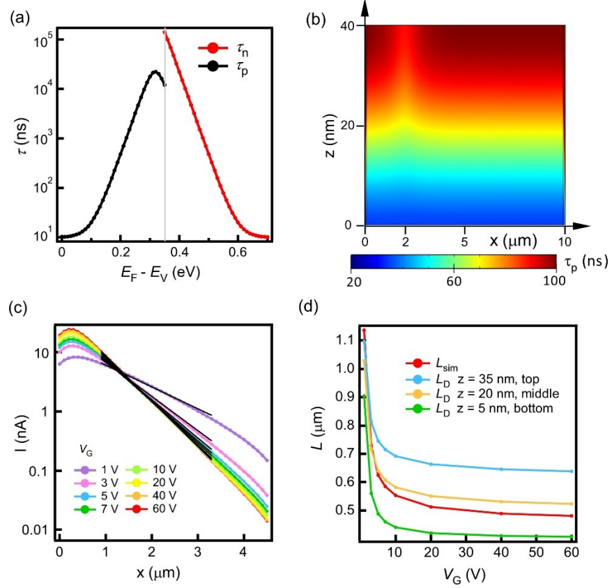
Figure 8. Photocurrent distributions simulated with n -dependent lifetime at V_{\text{SD}} = 0 V. (a) Electron and hole lifetimes as function of E_F . The grey vertical line indicates the mid-gap. (b) \tau_p distribution in the thin film channel with I_{\text{ex}} = 0.8 W/cm 2 at x = 2 \mu\text{m} and V_G = 10 V. (c) Photocurrent as a function of photoexcitation position at various V_G . The black curves are exponential fittings. (d) V_G dependent L_{\text{sim}} extracted from (c) and L_D calculated from \tau_p at different z .
