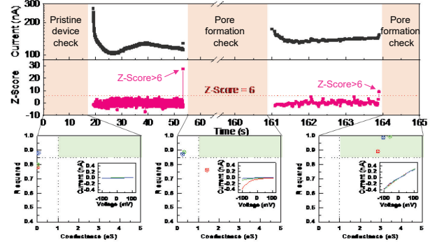
Figure 6: Top panel shows the current time-trace (black) under constant voltage stress with corresponding moving Z-Score (pink). Bottom panel shows scatter plots of membrane conductance and r^2 from the IV scanings.
