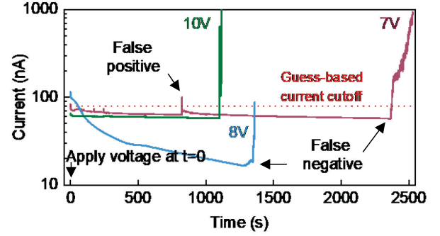
Figure 2: Leakage current time-traces at different DC voltages.
