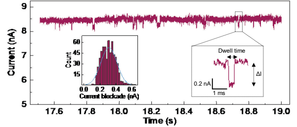
Figure 10: A representative current time-trace during the passage of DNA molecules through a nanopore.
