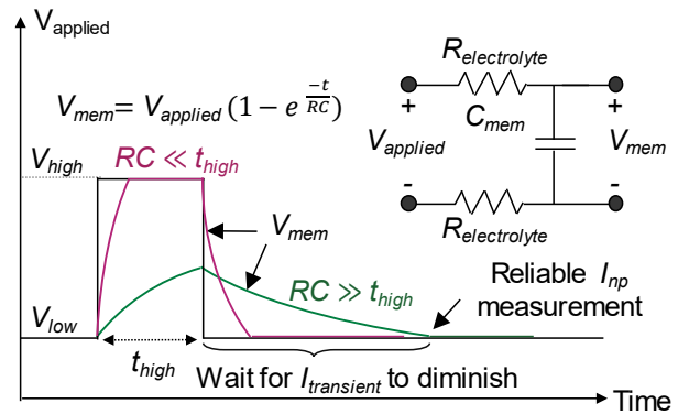
Figure 3: Membrane capacitance results in RC-dependent transmembrane voltage and transient current.
