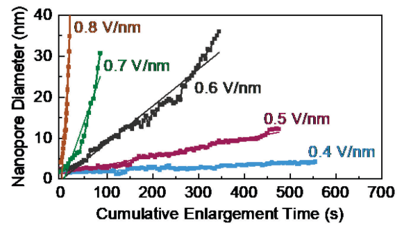
Figure 7: Nanopore diameter as a function of the cumulative enlargement time at various electric fields.
