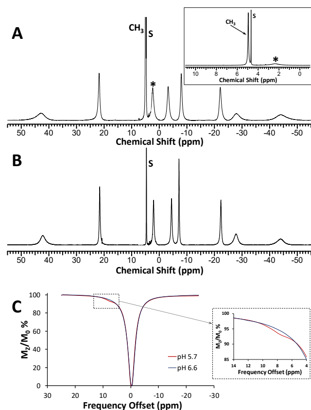
Figure 2. ^1\text{H} NMR spectra of A) [\text{Fe}(\text{Mim})]^{3+} in \text{D}_2\text{O} at pD 6.5 with inset showing expanded diamagnetic region, and B) [\text{Fe}(\text{Tim})]^{3+} in \text{D}_2\text{O} at pD 4.8, 25 ^\circ\text{C} . * – The intensity of this proton resonance of [\text{Fe}(\text{Mim})]^{3+} demonstrates the difference in scales. The solvent peak is labeled “S”. C) CEST effect of 25 mM \text{Fe}(\text{Tim}) observed at pH 5.7, 25 ^\circ\text{C} . Conditions: 40 mM MES, 100 mM NaCl in \text{H}_2\text{O} .
