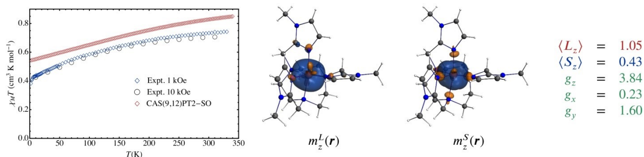
Figure 6. Calculated magnetic susceptibility \chi_M T ( \text{cm}^3 \text{K mol}^{-1} ) as a function of T (K) for [Fe(Mim)] 3+ . CAS(9,12)PT2-SO Results. Orbital ( m_z^L ) and spin ( m_z^S ) magnetization densities and g-factors for the ground-state doublet. Doublet components with \langle S_z \rangle > 0 . Iso-surfaces values \pm 0.001 au.
