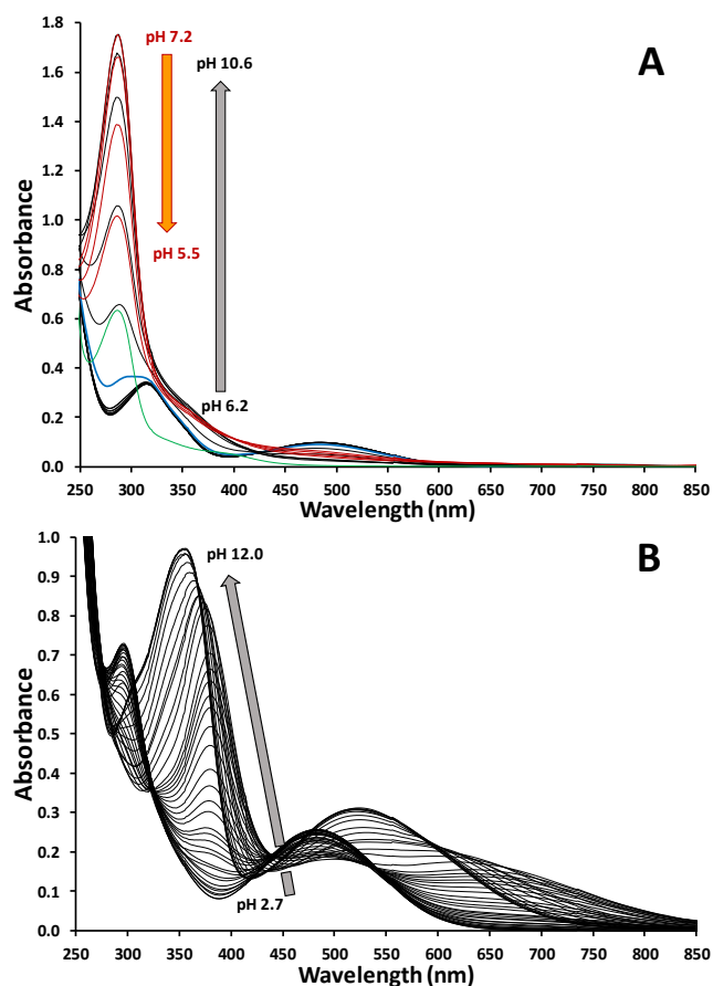
Figure 3. The pH-dependence of the UV-vis spectra of A) 0.86 mM \text{Fe}(\text{Mim}) at \text{pH} \leq 10.6 , where green line represents pure Mim (black lines – titration from pH 6.2 to pH 10.6; red lines – titration from pH 10.6 to pH 5.5; and B) 0.34 mM \text{Fe}(\text{Tim}) at pH 2.7 – pH 12.0. Conditions: 20 mM MES, 100 mM NaCl in \text{H}_2\text{O} at 37 °C. \text{pK}_{\text{a}1} 6.7, \text{pK}_{\text{a}2} 8.4, and \text{pK}_{\text{a}3} 9.7 are obtained from the fit.
