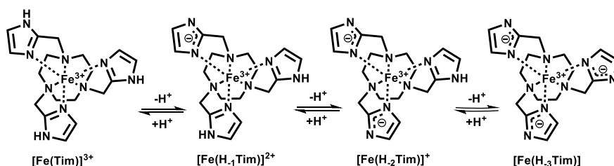
Scheme 2. pH-dependent speciation of the [\text{Fe}(\text{Tim})]^{3+} complex.
