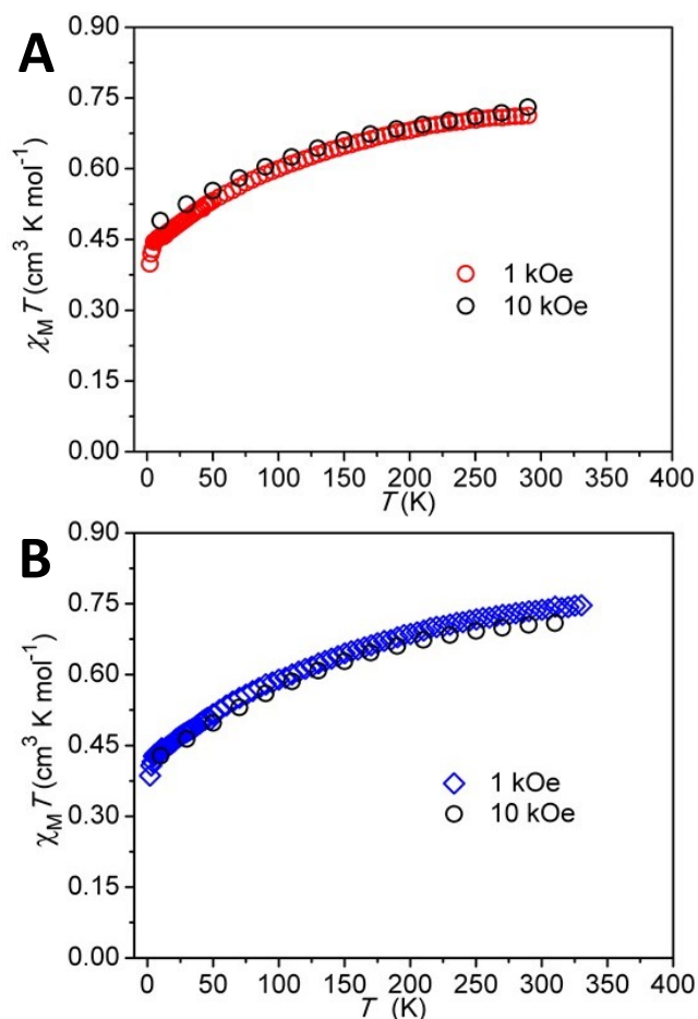
Figure 5. Temperature dependence of magnetic susceptibility for solid samples of A) [Fe( Tim )](OTf) 3 and B) [Fe( Mim )](OTf) 3 collected at applied fields of 1000 and 10000 Oe.
