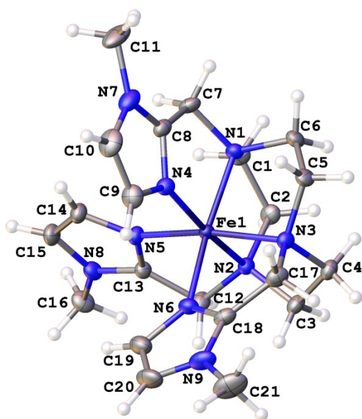
Figure 1. The ORTEP molecular structure of the [\text{Fe}(\text{Mim})]^{3+} cation, showing the atom-labeling scheme and 50% probability displacement ellipsoids.
